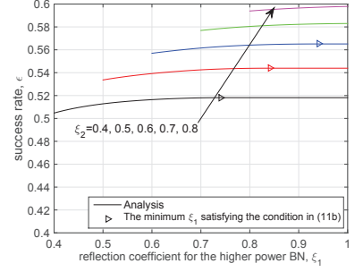
Fig. 4. Success rate \epsilon versus the reflection coefficient of the higher power BN \xi_1 under \alpha = 4 , m = 1 , P_T = 40 dBm and \gamma = 0 dB.
