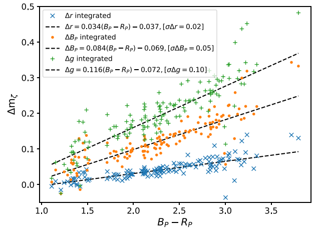
Figure 5. Gaia B_p , and SkyMapper gr systematic offsets between integrated flux-calibrated WiFeS spectra and MARCS model integrated spectra at literature parameters for our standard stars, plotted as a function of observed Gaia B_p - R_p . Stars redder in B_p - R_p have systematically more flux at bluer wavelengths, with the best-fitting linear magnitude offset plotted for each filter, and the standard deviation in magnitude noted.
