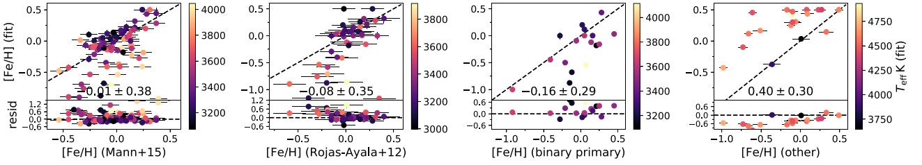
Figure 6. [Fe/H] recovery for our three-parameter fit in T_{\text{eff}} , [Fe/H], and m_{\text{bol}} for our four sets of [Fe/H] standards: Mann et al. (2015), Rojas-Ayala et al. (2012), primary star [Fe/H] for cool dwarfs in binaries, and mid-K dwarfs. The median and standard deviation of each set of residuals are annotated. Note the inability of the three-parameter fit to reliably recover [Fe/H], with the scatter on our recovered [Fe/H] for the binary sample (the most reliable set of [Fe/H] standards) being larger than the scatter on our photometric [Fe/H] relation.
