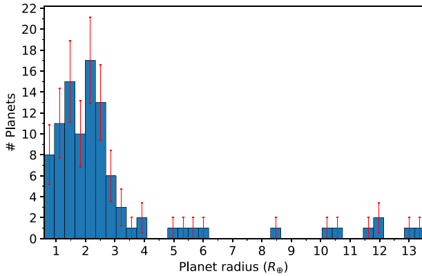
Figure 12. Histogram of candidate planet radii with R_P < 14 R_\oplus , with 0.35 R_\oplus width bins and Poisson uncertainties. Note that we detect the exoplanet radius gap at an \sim 1\sigma level, though remain limited by our small sample size.
