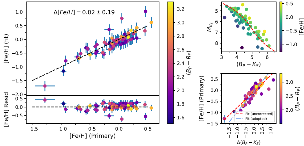
Figure 3. Left: Cool dwarf secondary [Fe/H] calculated from our photometric calibration versus [Fe/H] from the associated FGK primary star, colour coded by Gaia ( B_p - R_p ). The standard deviation of the residuals, and our adopted uncertainty for the relation, is \pm 0.19 dex. See Table C1 for further information on this FGK–KM binary calibration sample. Top Right: M_{K_S} - (B_p - K_S) colour–magnitude diagram for the calibration sample of cool dwarf secondaries colour coded by host star [Fe/H]. The dashed red line is a third-order polynomial representing the main sequence, fitted to the Mann et al. (2015) sample of cool dwarfs. Bottom right: Fitted [Fe/H] as a function \Delta(B_p - K_S) offset from the mean main sequence polynomial. The dashed red line is the initial uncorrected linear least-squares fit, and the dash–dotted blue line is the adopted fit after correcting for the remaining trend in the residuals.
