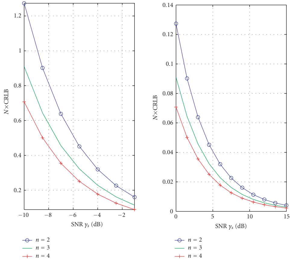
FIGURE 1: CRLB versus symbol SNR \gamma_s for n -order monocycles with t_p = 2 nanoseconds; n = 2, 3, 4 .
