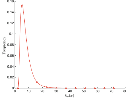
Fig. 2. Normalized histogram of \kappa_o(x) of a flat surface. Pixels with \kappa_o(x) \rightarrow \infty (due to amplitude and phase) have been scaled down to finite values. The heavy tail is associated with noisy data.
