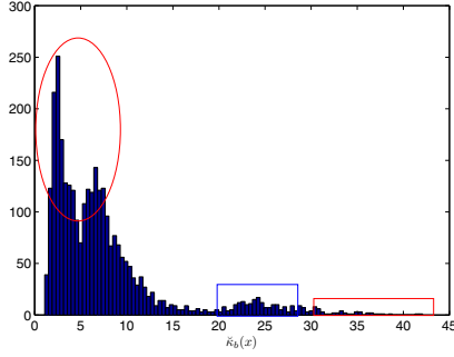
Fig. 4. Histogram of a \kappa_b(x) for a single frame
