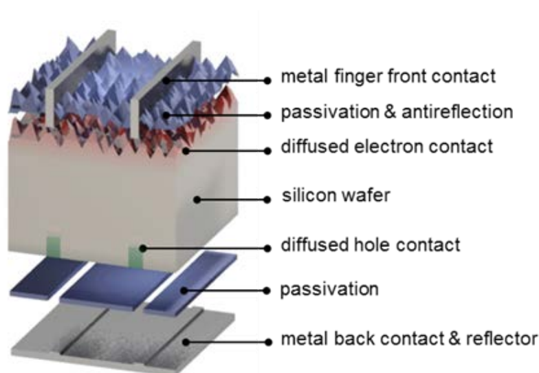
Fig. 6: Schematic of the components of a localized rear contact solar cell with dielectric rear surface passivation. Aluminum doping from the back contact into the silicon wafer (green) is confined to the small openings in the rear passivation layer, minimizing recombination. The dielectric passivation layer simultaneously improves the reflectivity of the aluminum back reflector.
