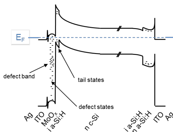
Fig. 10: Energy band diagram of a \text{MoO}_x - silicon heterojunction solar cell in equilibrium. Comparison with Fig. 9 reveals that n-type \text{MoO}_x has an effect similar to that of p-type amorphous silicon on band bending in the crystalline silicon absorber due to its high work function. Representative values were used for the modelling of the curves with the program PC1D 66 (n-type crystalline silicon wafer doped with 1 \cdot 10^{15} \text{ cm}^{-3} electrons, amorphous silicon with a band gap of 1.8 eV and electron concentration of 1 \cdot 10^{19} \text{ cm}^{-3} for the n-type amorphous silicon; for \text{MoO}_x and ITO, a band gap of 3.3 eV and an electron concentration of 1 \cdot 10^{16} and 1 \cdot 10^{21} \text{ cm}^{-3} were assumed). Layer thicknesses along the horizontal axis are not to scale for readability. In particular, the depletion region extends about 1.5 \mu\text{m} into the crystalline silicon wafer.
