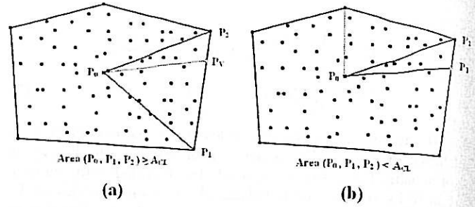
Figure 1: An example of clustering procedure, P_0 is the centroid location of sensing field, P_1 and P_2 are the locations of two boundary sensor nodes, P_V \in \overline{P_1 P_2} , and A_{CL} is the cluster area.
