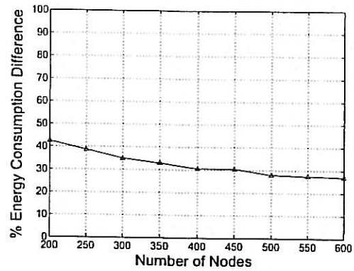
Figure 11: The minimum and maximum energy consumption differences among the cluster heads as the number of network sensor nodes are varied.
