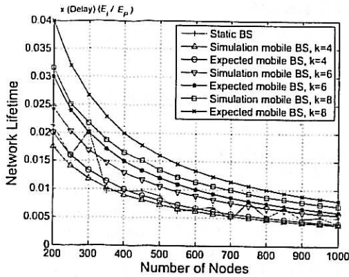
Figure 10: Network lifetime as it varies with the number of network sensor nodes, for static and mobile BSs with different k .
