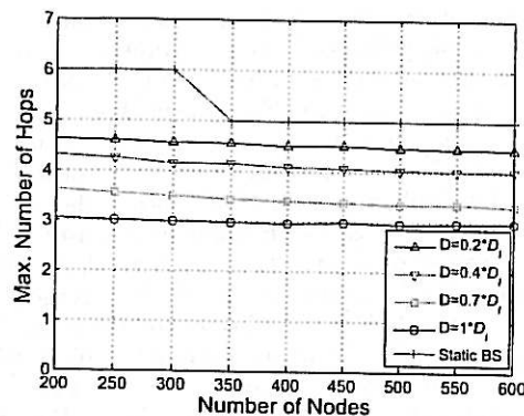
Figure 13: The maximum number of hops as it varies with the number of network sensor nodes, for static and mobile BSs.
