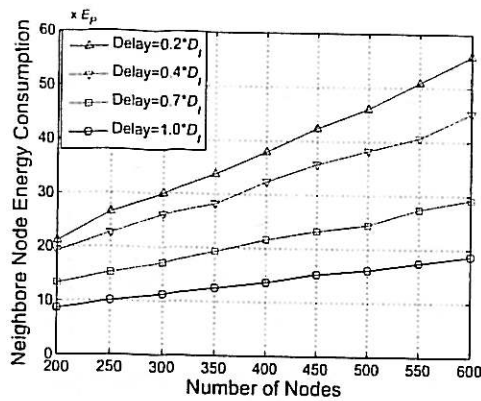
Figure 12: The minimum cluster head neighboring sensor nodes energy consumption as the number of network sensor nodes are varied, for various data gathering delay.
