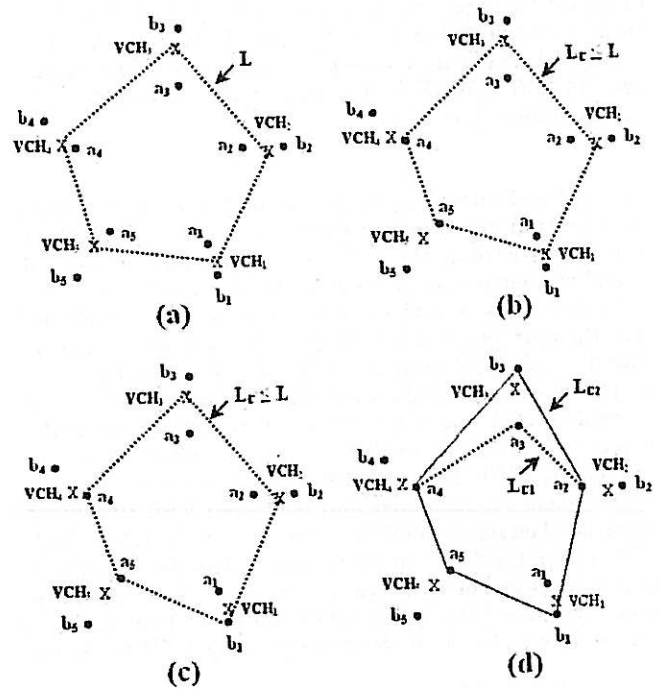
Figure 9: An execution example of finding real cluster heads, k = 5 . (a) Finding two candidate cluster heads for each cluster, one with RS_i \geq VS_i and the other with RS_i < VS_i , 1 \leq i \leq k . (b) After the execution of Phase I, sensor nodes a_4 and a_5 are elected as real cluster heads since they are closest to VCH_4 , VCH_5 and RS_4 < VS_4 , RS_5 < VS_5 , respectively. (c) Then, sensor node b_1 is elected as real cluster head since it is closest to VCH_1 and L_c \leq L . (d) After the execution of Phase II, sensor nodes a_2 and a_3 are initially elected as real cluster heads, then a_3 is changed with b_3 as real cluster head since it is closest to VCH_3 and L_{c2} \leq L , b_2 is not elected as real cluster head since the corresponding BS tour length is greater than L .
