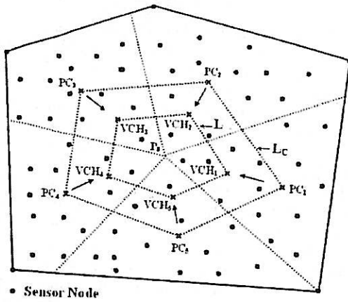
Figure 4: An illustrative example of virtual cluster heads calculation, for k = 5 . Sensor nodes are denoted by black circles. PC_i , 1 \leq i \leq k are the locations of clusters area center points and VCH_i , 1 \leq i \leq k are the virtual cluster heads. L_C and L are the BS tour length connecting PC_i and VCH_i , respectively. L < L_C .
