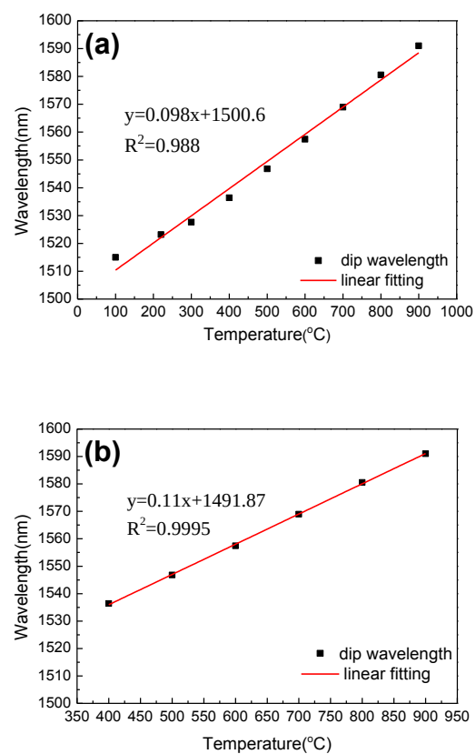
Fig.7. The relationships between dip wavelength and temperature. (a) temperature ranges from 100 °C to 900 °C and (b) temperature ranges from 400 °C to 900 °C.
