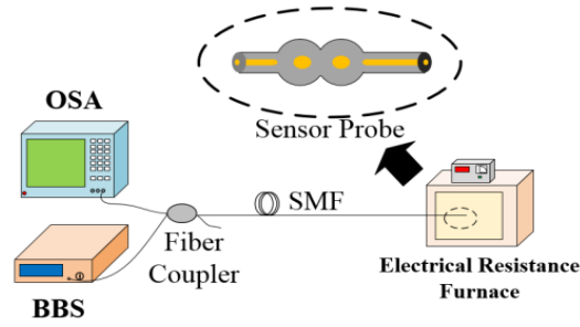
Fig.1. System configuration for experimental setup of high-temperature measurement with peanut flat-end reflection structure.
