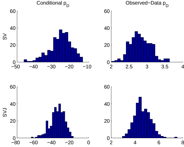
Figure 4: The effective number of parameters p_D computed using the conditional and observed-data likelihoods.
