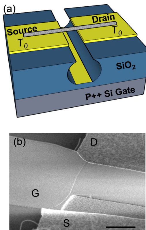
FIG. 1. (Color online) (a) Schematic drawing of our suspended SWNT devices with 10 nm W/20 nm Pt leads. (b) Scanning electron microscopy image of a typical suspended device over \sim 2 \mu\text{m} trench. Scale bar is 1 \mu\text{m} .
