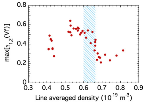
Figure 7. Maximum value of the cross-correlation between floating potential signals measured at approximately the same radial positions of both probes ( \rho \approx 0.9 ) as a function of plasma density. As in figure 6, the shaded area corresponds to the critical density.
