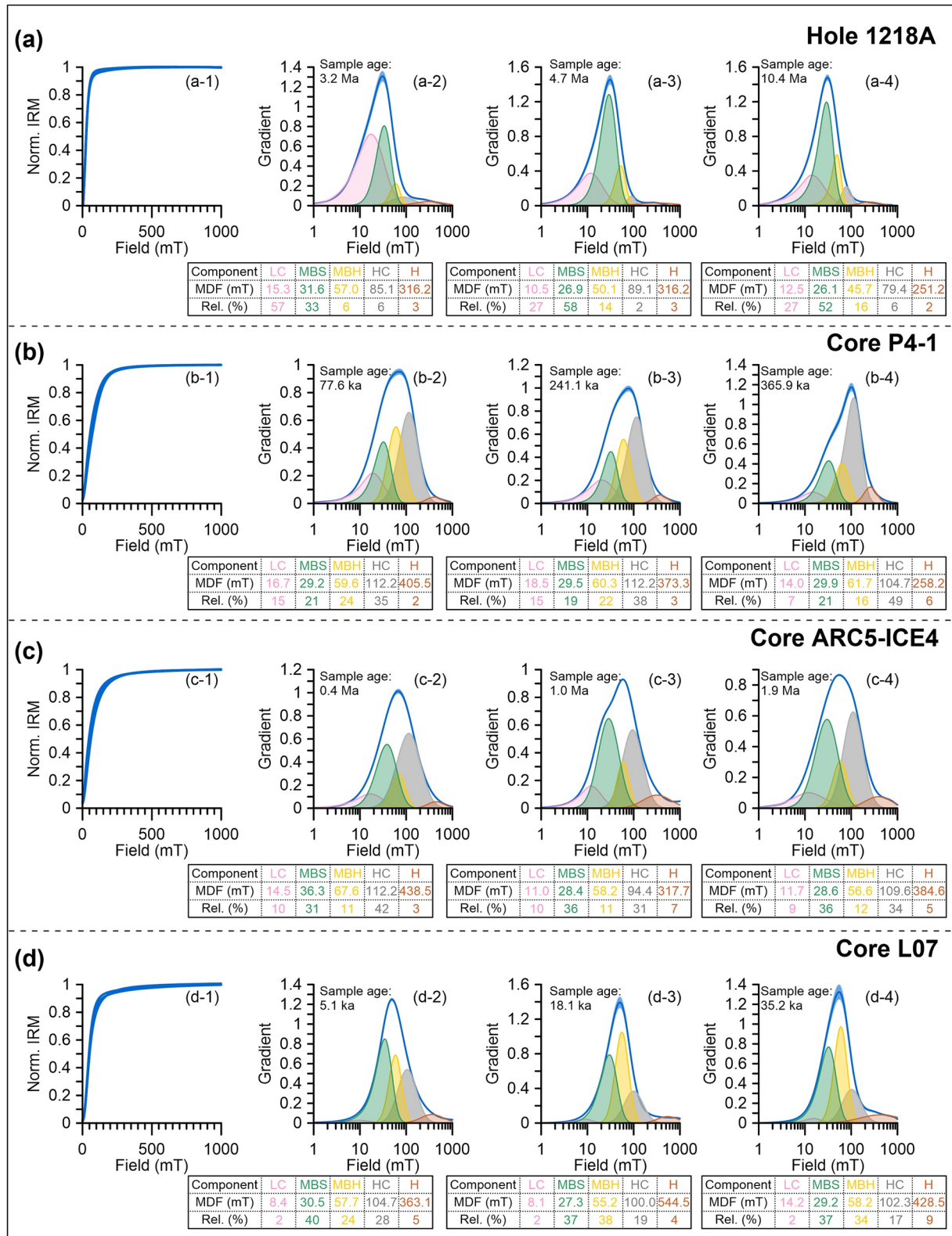
Figure 6. IRM unmixing results. The data were analyzed using the MAG-MIX software (CODICA and GECA). (a-1 to d-1) Normalized IRM acquisition curves. (a-2 to a-4, b-2 to b-4, c-2 to c-4, and d-2 to d-4) Coercivity distributions of IRM. The low-coercivity (LC), MBS, MBH, high-coercivity (HC), and hematite (H) components are labelled with pink, green, yellow, gray, and brown, respectively. The sum of coercivity distributions (blue) are plotted together with their confidence limits. The median destructive field (MDF) and relative contribution (Rel.) are shown in the respective tables.
