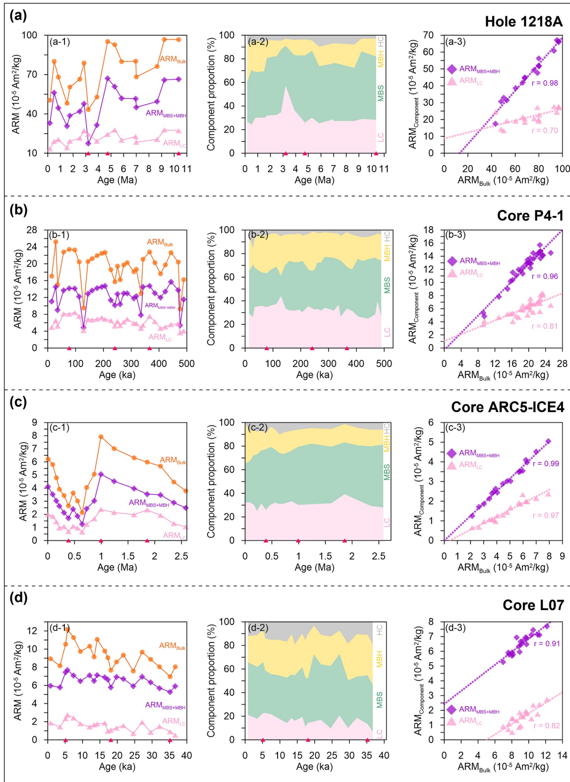
Figure 2. Comparison between ARM component analysis results and bulk ARM ( ARM_{Bulk} ). (a-1 to d-1) Variation of ARM_{Bulk} , ARM carried by MBS + MBH ( ARM_{MBS+MBH} ), and low-coercivity ( ARM_{LC} ) components. (a-2 to d-2) Variations of component proportions obtained from ARM coercivity spectra. (a-3 to d-3) Correlation plots of ARM_{MBS+MBH} versus ARM_{Bulk} and ARM_{LC} versus ARM_{Bulk} . The correlation coefficient is r . Red triangles on the age axis indicate samples for which FORC diagrams are shown in Figure 5.
