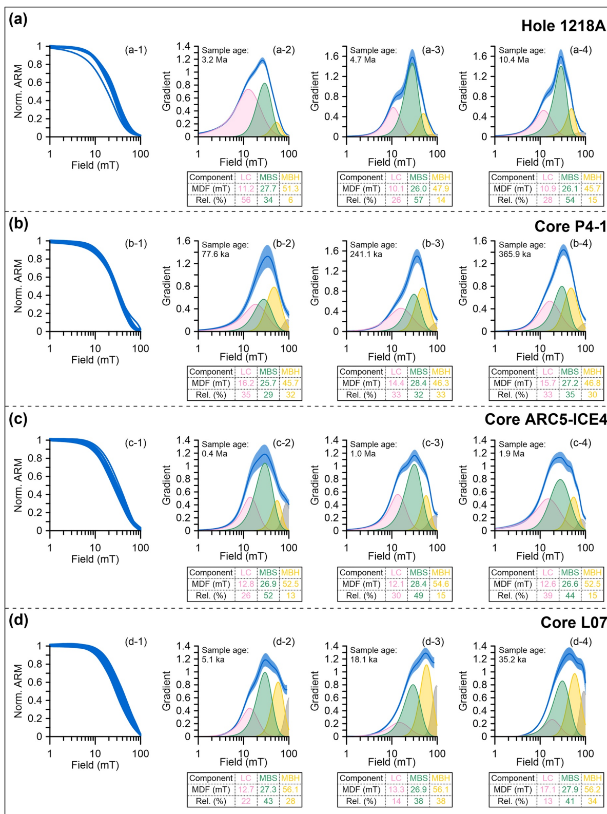
Figure 3. ARM component analysis results. The data were analyzed using the MAG-MIX software (CODICA and GECA). (a-1 to d-1) Normalized ARM demagnetization curves. (a-2 to a-4, b-2 to b-4, c-2 to c-4, d-2 to d-4) Coercivity distributions of ARM. The low-coercivity (LC), MBS, MBH, and high-coercivity (HC) components are labelled with pink, green, yellow, and gray, respectively. The sum coercivity distributions (blue) are plotted together with their confidence limits. The median destructive field (MDF) and relative contribution (Rel.) are shown in the respective tables. Information for HC is not shown here due to its incomplete definition due to the limited maximum AF used.
