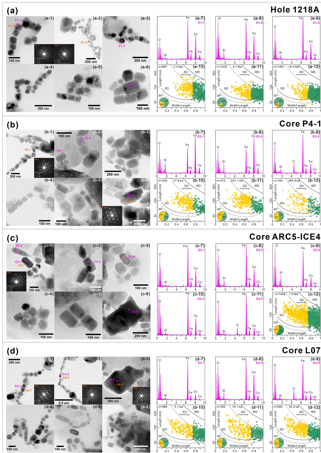
Figure 4. Transmission electron microscope (TEM) images for (a) Hole 1218A, and cores (b) P4-1, (c) ARC5-ICE4, and (d) L07. TEM images are shown in a-1 to a-6, b-1 to b-6, c-1 to c-6, and d-1 to d-6. Insets are selected area electron diffraction (SAED) patterns for the corresponding analysis points. Respective energy-dispersive X-ray spectroscopy (EDXS) results are shown in a-7 to a-9, b-7 to b-9, c-7 to c-9, and d-7 to d-9. Si and Cu signals are from nearby silicate particles and Cu grid, respectively. Magnetofossil size distributions are shown in a-10 to a-12, b-10 to b-12, c-10 to c-12, and d-10 to d-12, where yellow and green symbols denote magnetofossils with elongated ( \text{width/length} < 0.75 ) and equant ( 0.75 < \text{width/length} < 1 ) crystals, respectively (Kopp & Kirschvink, 2008); pie charts are the corresponding statistics.
