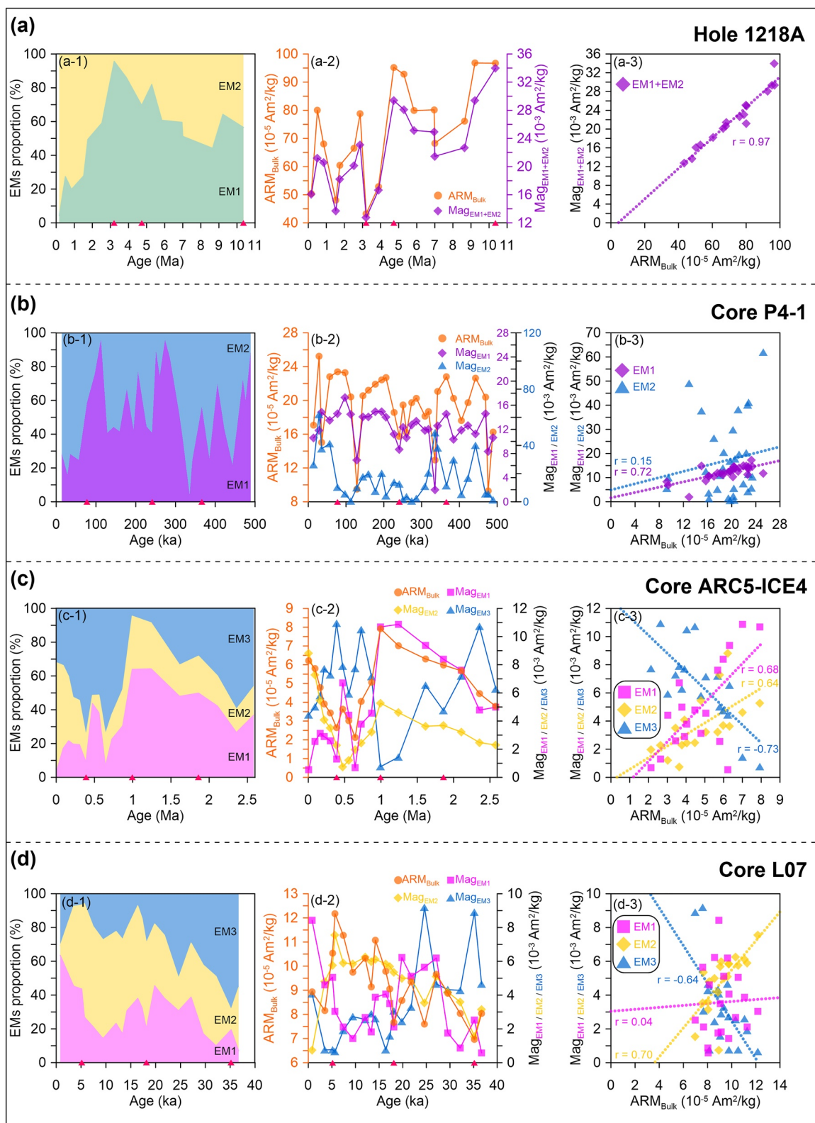
Figure 8. Comparison between ARM and FORC-PCA results. (a-1 to d-1) Variations of EM proportions obtained from FORC-PCA. (a-2 to d-2) Variations of ARM_{Bulk} and magnetization ( Mag ) carried by EMs from FORC-PCA. (a-3 to d-3) Correlation diagrams between EM magnetizations and ARM_{Bulk} . The correlation coefficient is r . Red triangles on the age axis indicate samples for which FORC diagrams are shown in Figure 5.
