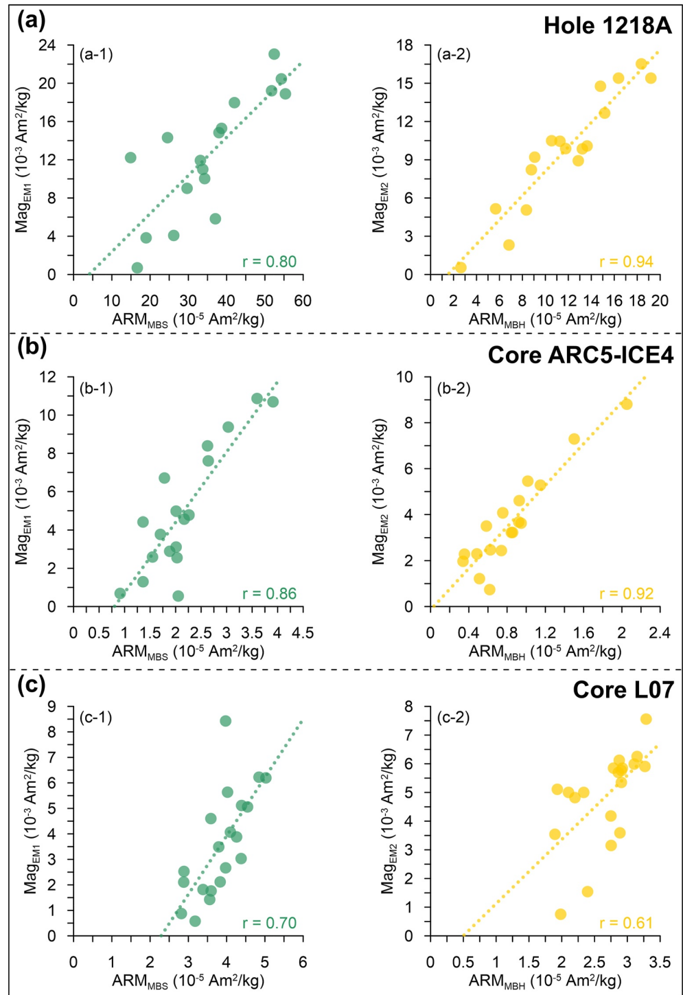
Figure 9. Comparison between ARM components and FORC-PCA endmembers. All horizontal axes represent the ARM carried by either MBS or MBH from ARM component analysis. All vertical axes represent the magnetization carried by EMs identified from FORC-PCA. The correlation coefficient is r .
