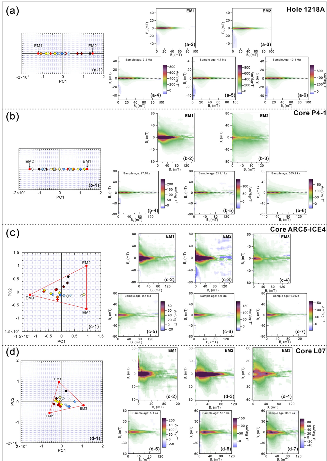
Figure 5. FORC-PCA results for (a) Hole 1218A (VARIFORC (Egli, 2013) smoothing parameters are: S_{c0} = 4 , S_{b0} = 3 , and S_{c1} = S_{b1} = 7 ); (b) core P4-1 ( S_{c0} = 4 , S_{b0} = 3 , and S_{c1} = S_{b1} = 7 ); (c) core ARC5-ICE4 ( S_{c0} = 5 , S_{b0} = 4 , and S_{c1} = S_{b1} = 7 ); and (d) core L07 ( S_{c0} = 6 , S_{b0} = 5 , and S_{c1} = S_{b1} = 9 ). Principal component (PC) scores are shown for the samples in a-1 to d-1. End member (EM) FORC diagrams are shown in a-2, a-3, b-2, b-3, c-2, c-3, c-4, d-2, d-3, and d-4. FORC diagrams for representative samples are shown in a-4 to a-6, b-4 to b-6, c-5 to c-7, and d-5 to d-7.
