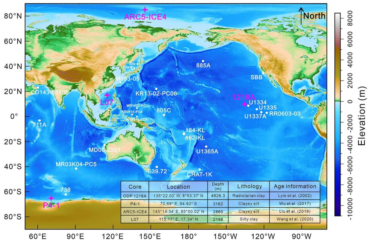
Figure 1. Location map of cores studied here. Also shown are sites from which magnetofossil records have been reported, including Sites 4 and 6 (Yamazaki et al., 2019), core KR13-02-PC06 (Yamazaki et al., 2020), IODP Hole U1365A (Yamazaki & Shimono, 2013), cores KR0515-PC2 and PC4 (Yamazaki & Horiuchi, 2016), core MR1402-PC1 (Sakuramoto et al., 2017), ODP Hole 805C (Tarduno et al., 1998), cores 182/184-KL (Vali et al., 1987), core MD00-2361 (Heslop et al., 2013), core M063-05 (Li et al., 2019), core E39.72 (Hesse, 1994), core CHAT-1K (Lean & McCave, 1998), IODP Sites U1334 and U1335 (Channell et al., 2013), IODP Hole U1337A (Yamazaki, 2012), core RR0603-03 (Chen et al., 2017), Site SBB (Santa Barbara Basin) (Stolz et al., 1986), core CD143-55705 (Chang, Heslop, et al., 2016), ODP Hole 711A (Chang et al., 2012), core MR03K04-PC5 (Yamazaki & Ikehara, 2012), ODP Site 738 (Larrasoana et al., 2012; Roberts et al., 2011), and ODP Hole 885A (Zhang et al., 2021). Details of the studied cores are indicated in the inset table.
