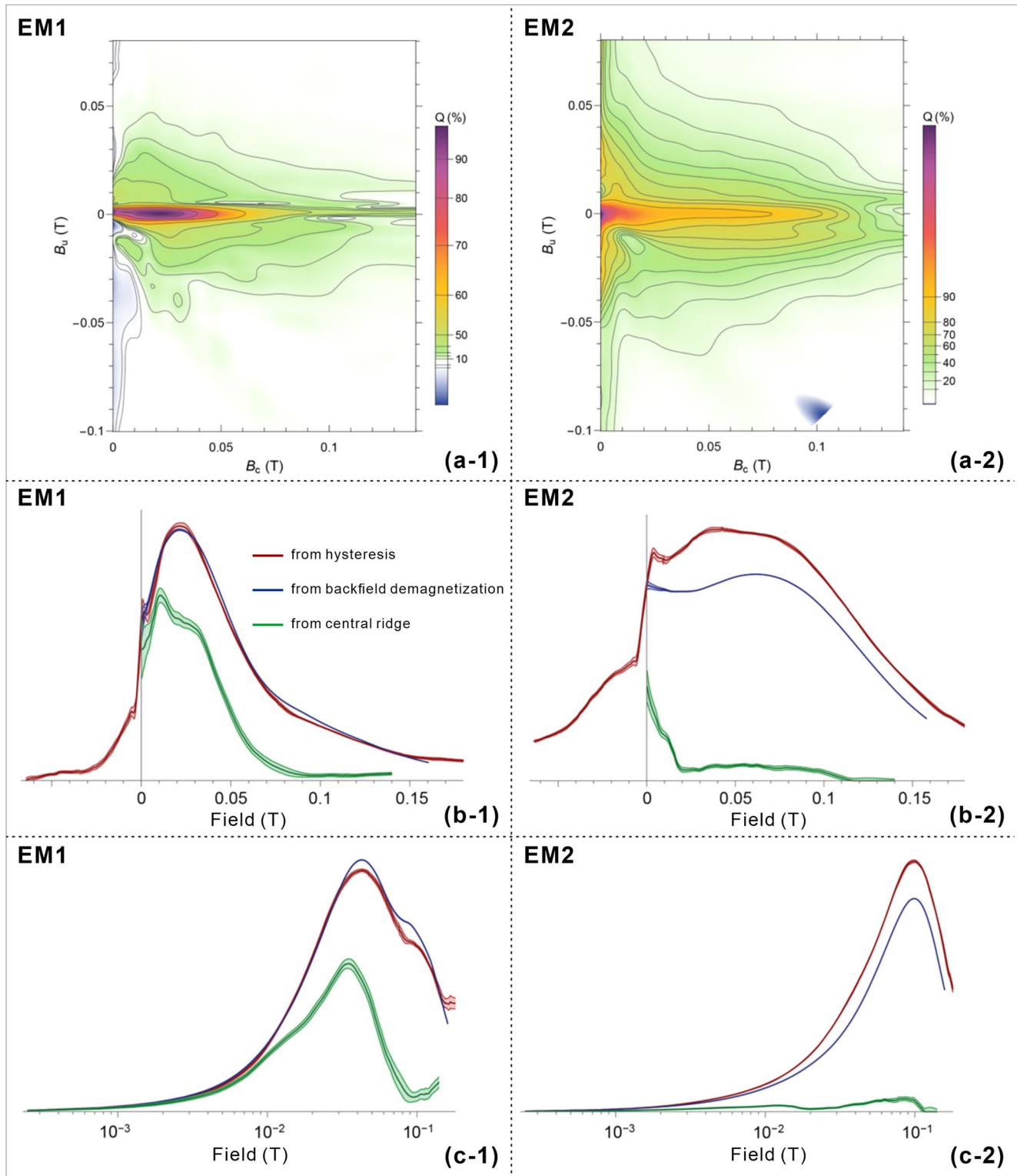
Figure 10. Quantitative FORC EM analyses for core P4-1 based on quantile contours (a-1 and a-2) and coercivity distributions (b-1, b-2, c-1, c-2). Coercivity distributions plotted on a (b-1 and b-2) linear field scale and (c-1 and c-2) logarithmic field scale. Bulk EM properties can be obtained: EM1: M_{rs}/M_s = 0.356 , M_c/M_{rs} = 0.471 , and non-central ridge contributions (52.9%) are only slightly asymmetric and reflect the central ridge coercivity distribution. EM2: M_{rs}/M_s = 0.224 , M_c/M_{rs} = 0.072 , and non-central ridge contributions (92.8%) dominate with a significant HC fraction.
