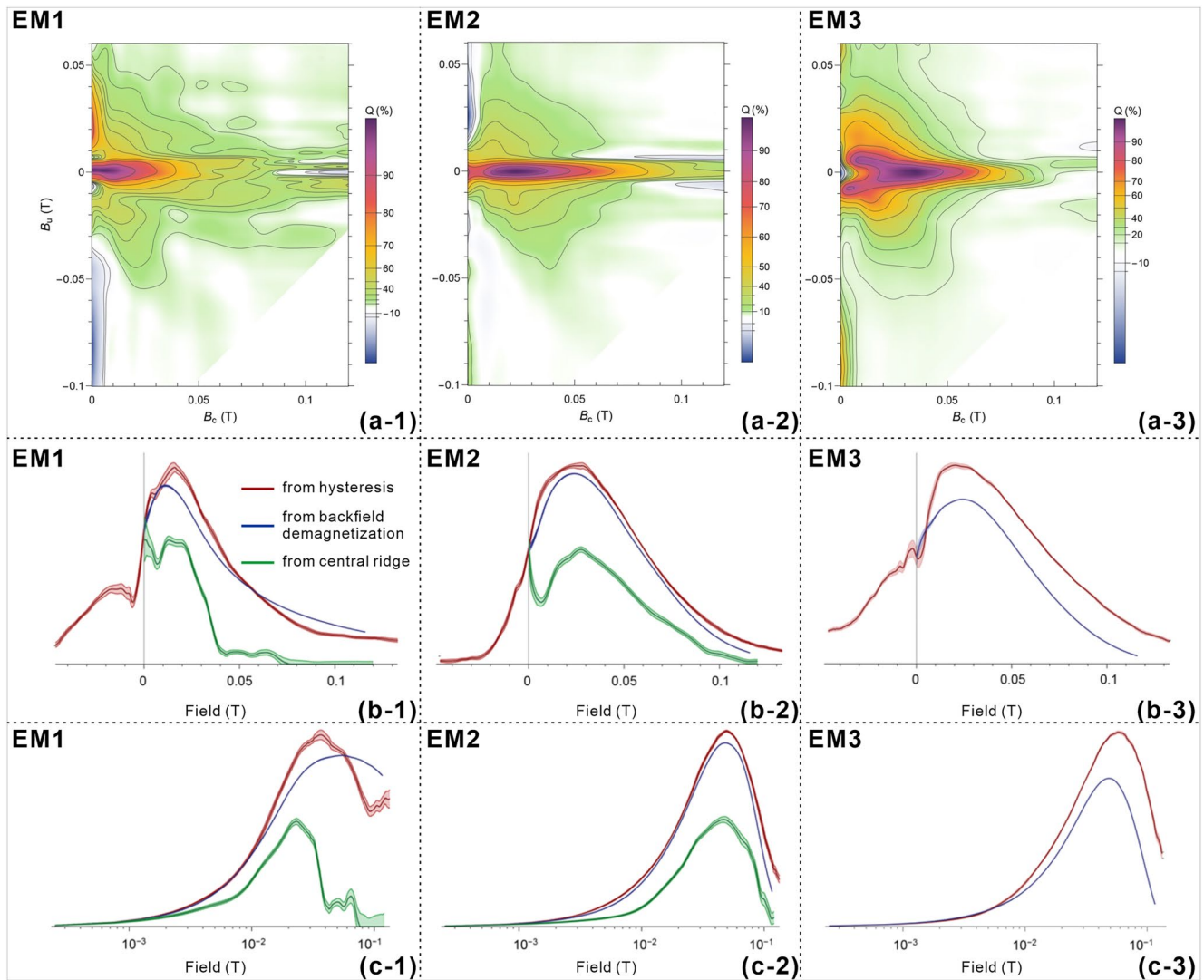
Figure 12. Quantitative analyses of FORC EMs for core L07 based on quantile contours (a-1, a-2, and a-3) and coercivity distributions (b-1, b-2, b-3, c-1, c-2, c-3). Coercivity distributions plotted on (b-1, b-2, and b-3) linear and (c-1, c-2, and c-3) logarithmic field scales. Bulk EM properties can be obtained: EM1: M_{rs}/M_s = 0.286 , M_c/M_{rs} = 0.328 , and non-central ridge contributions (67.2%; noisy and affected by unmixing artifacts). EM2: M_{rs}/M_s = 0.324 , M_c/M_{rs} = 0.543 , and non-central ridge contributions (45.7%; noisy and affected by slight unmixing artifacts). EM3: M_{rs}/M_s = 0.197 , M_c/M_{rs} = 0 , and unmixing artifact near the origin.
