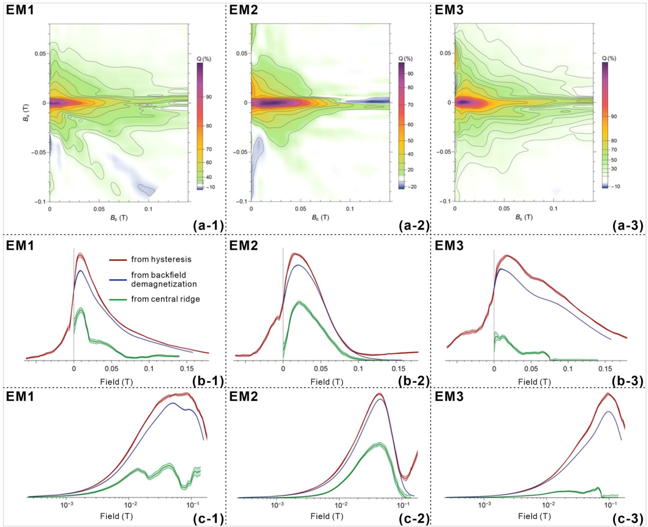
Figure 11. Quantitative analyses of FORC EMs for core ARC5-ICE4 based on quantile contours (a-1, a-2, and a-3) and coercivity distributions (b-1, b-2, b-3, c-1, c-2, c-3). Coercivity distributions plotted on (b-1, b-2, and b-3) linear and (c-1, c-2, and c-3) logarithmic field scales. Bulk EM properties can be obtained: EM1: M_{rs}/M_s = 0.286 , M_{cr}/M_{rs} = 0.327 , and non-central ridge contributions (67.3%, noisy). EM2: M_{rs}/M_s = 0.290 , M_{cr}/M_{rs} = 0.486 , and non-central ridge contributions (51.4%) are asymmetric with upper quadrant termination at \sim 55 mT, similar to the magnetofossil signature calculated by Amor et al. (2022), with unmixing artifact along the central ridge above 100 mT. EM3: M_{rs}/M_s = 0.225 , M_{cr}/M_{rs} = 0.111 , and non-central ridge contributions (88.9%) over the upper and lower quadrant are nearly symmetric.
