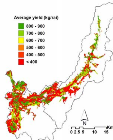
Figure 6. Estimated yield map simulated by BN approach
