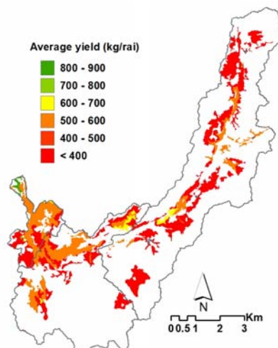
Figure 5. Estimated yield map simulated by fuzzy approach
