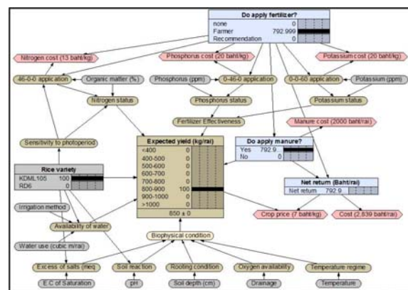
Figure 3. The probability approach crop-economic model
