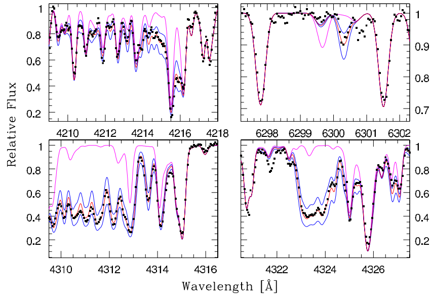
Figure 1. Observed and synthetic spectra around CH-bandheads (lower panels), CN-band (upper left panel) and O line (upper right panel) for the star 248664. The magenta line is the spectrum computed with no contribution from C, N, and O; the red lines and blue lines are the best-fitting and the syntheses computed with abundance altered by \pm 0.25 dex from the best value, respectively.
