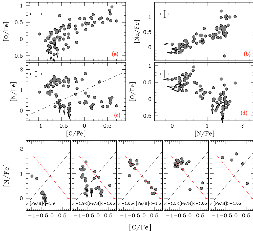
Figure 2. Upper panels: [N/Fe] and [O/Fe] vs. [C/Fe] (panels (c), (a)), and [O/Fe] and [Na/Fe] vs. [N/Fe] (panels (d), (b)). The dashed black line in panel (c) separates C-poor/N-rich stars from C-rich/N-poor ones. Lower panels: [N/Fe] vs. [C/Fe] in metallicity bins defined in Marino et al. (2011a). In each panel, the dashed black line is the same as in panel (c), the red dot-dashed line represents the “best-fit” line of constant [C/Fe] + [N/Fe] (=0.80) for the mid-metallicity stars.
