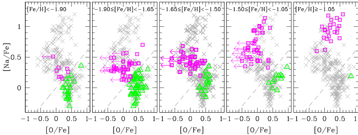
Figure 4. Our adopted division of stars in O-rich/Na-poor (first generation) and O-poor/Na-rich ones (second generation) has been represented in the Na-O plane for each metallicity bin, as quoted in the insets. The dashed line separates the selected first-generation stars represented by green triangles, and from the selected second-generation stars represented by magenta squares. Gray crosses in each panel represent the entire sample analyzed by Marino et al. (2011a).
