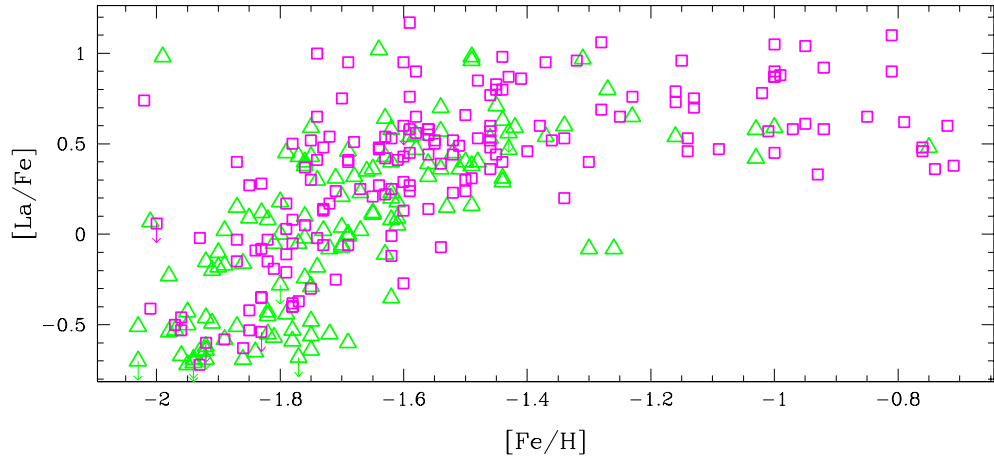
Figure 6. [\text{La}/\text{Fe}] as a function of [\text{Fe}/\text{H}] . Symbols are the same as in Figure 4.
