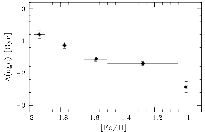
Figure 9. Age difference for each \omega Cen sub-population, between the estimates based on CNO-enhanced isochrones and on the actual C+N+O abundances, and the measurements provided by not CNO-enhanced isochrones.
