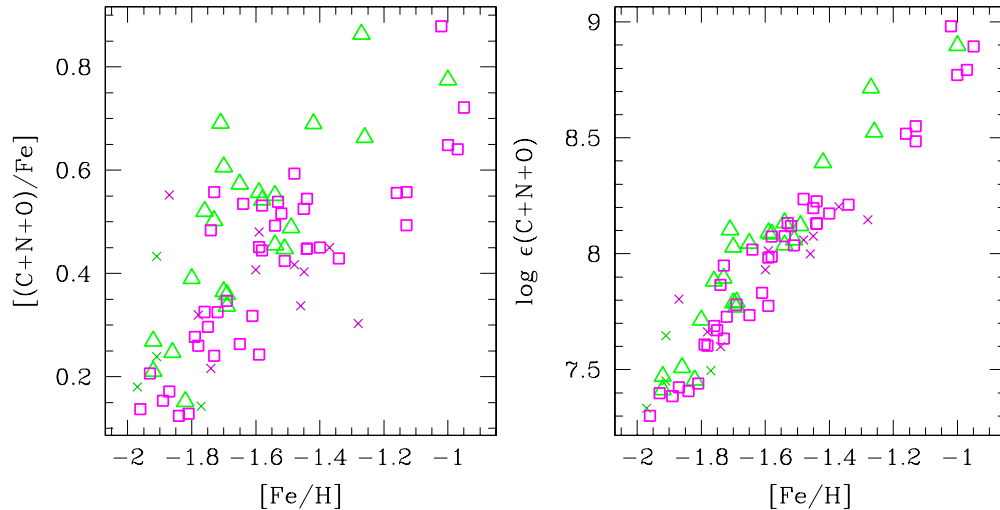
Figure 8. CNO relative to Fe and \log \epsilon(\text{CNO}) as a function of [\text{Fe}/\text{H}] . Symbols are the same as in Figure 4. Crosses mark stars for which we have only an upper limit for N or O.
