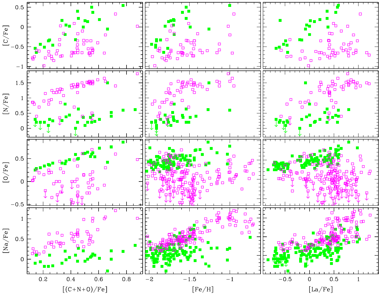
Figure 7. C, N, O, and Na abundance ratios as a function of [(\text{C}+\text{N}+\text{O})/\text{Fe}] , [\text{Fe}/\text{H}] , and [\text{La}/\text{Fe}] . Symbols are the same as in Figure 4.
