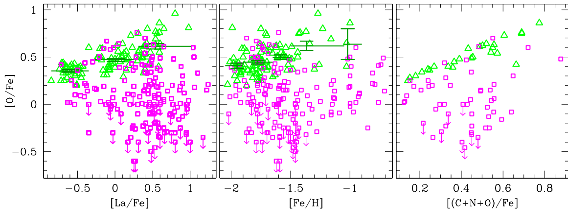
Figure 5. O abundance ratios as a function of [La/Fe] , [Fe/H] , and [(C+N+O)/Fe] . Symbols are the same as in Figure 4. The dark green vertical error bars represent the error associated with the mean [O/Fe] abundance in different intervals in [La/Fe] and [Fe/H] delimited by the horizontal line.
