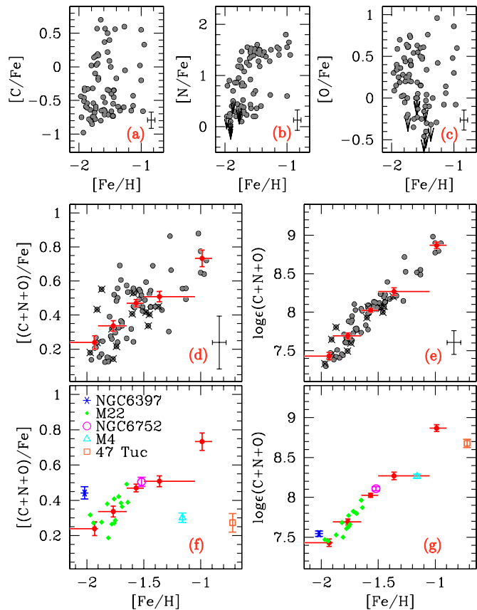
Figure 3. Upper panels: [C/Fe] , [N/Fe] , and [O/Fe] vs. [Fe/H] . Middle panels: [(C+N+O)/Fe] and \log\epsilon(C+N+O) vs. [Fe/H] . Stars with upper limits for O or N abundances are represented as gray crosses. Red points represent the average C+N+O content in the metallicity intervals spanned by the horizontal red bars. Vertical bars are the errors associated with the mean values. Lower panels: average [(C+N+O)/Fe] vs. iron for the GCs quoted in the inset compared with the \omega Cen CNO mean values (red points) of panels (d) and (e). Data for the mono-metallicity GCs are from Ivans et al. (1999) for M4, and Carretta et al. (2005) for 47 Tuc, NGC 6752, and NGC 6397. Data for M22 are from Marino et al. (2011b).
