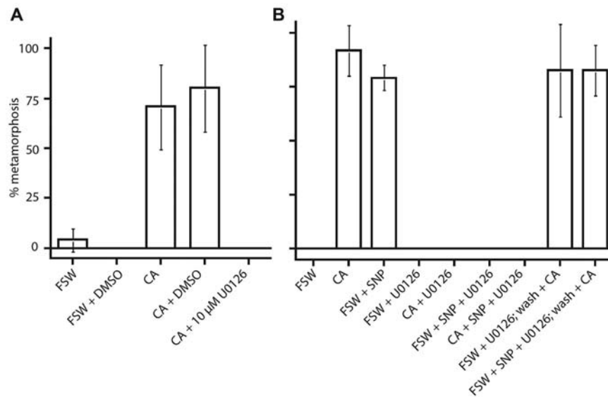
Figure 3. Inhibition of MAPK signalling prevents A. queenslandica metamorphosis. (A) Larvae subjected to 10 μM U0126 are inhibited from initiating metamorphosis, even in the presence of the inductive coralline algae; an equivalent concentration of 0.1% DMSO does not inhibit metamorphosis. (B) Larvae subjected to NO donor, 2.5 μM SNP, undergo metamorphosis at rates similar to coralline algae controls. MAPK inhibitor U0126 inhibits metamorphosis when larvae are in the presence of SNP, coralline algae or both. Larvae removed from U0126, washed in FSW and subjected to the inductive coralline algae undergo high rates of normal metamorphosis.
