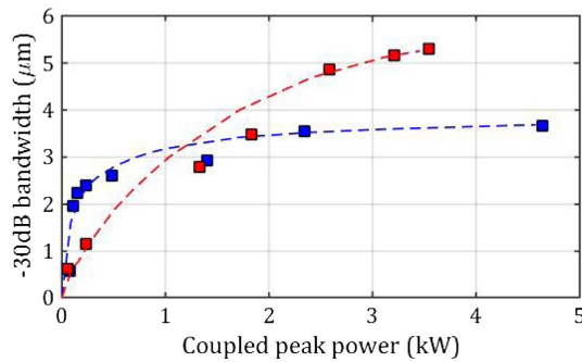
Fig. 8. Bandwidth at -30 dB versus coupled peak power experimentally measured for the waveguide (1) (blue) and waveguide (2) (red). The dashed curves are guides for the eye.
