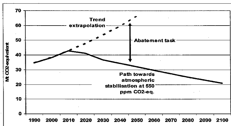
Figure 1: A pathway to Stable Greenhouse Gas Concentrations
