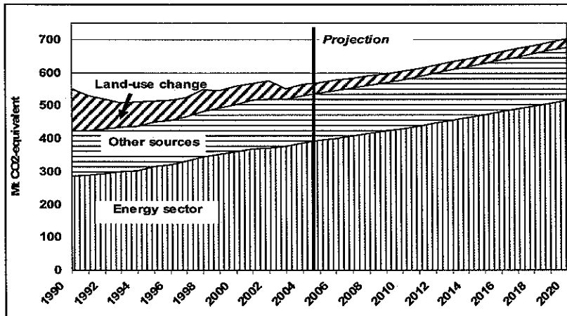
Figure 2: Australia's Greenhouse Gas Emissions
