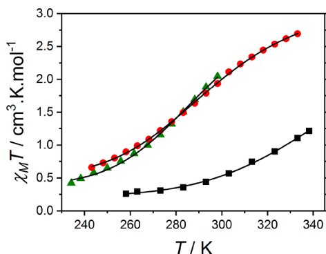
Figure 6. Plot of \chi_M T vs T for 1 + in MeCN solution (■), DCM solution (▲) and DCE solution (●). Solid black lines indicate fits to the regular solution model with parameters in Table 4.
