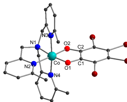
Figure 2. Structure of 1 + in 1 (PF 6 )·2tol. Color code: carbon, black; oxygen, red; nitrogen, blue; cobalt, aqua green; bromine, brown.
