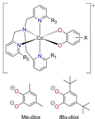
Figure 1. Family of complexes [\text{Co}(\text{Me}_n\text{tpa})(\text{Xdiox})]^+ ; \text{R}_1 , \text{R}_2 , and \text{R}_3 = \text{H} or \text{Me} ; \text{X} = \text{Br}_4 , \text{Cl}_4 , \text{H}_4 , 3,5- \text{Me}_2 , 3,5- t\text{Bu}_2 .
