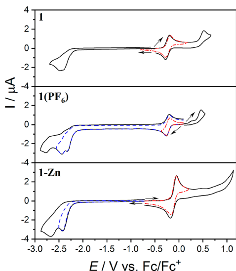
Figure 7. Cyclic voltammetry of DMF solutions (1.0 mM with 0.1 M \text{Bu}_4\text{NPF}_6 ) of compound 1 (top), 1 ( \text{PF}_6 ) (middle), and 1-Zn (bottom) obtained with a 1.0 mm diameter glassy carbon electrode at a scan rate of 100 \text{ mV s}^{-1} . The blue dashed and red dot-dashed lines plot the voltammograms measured with a switching potential immediately past the first reversible process or highly negative reduction, respectively. Arrows indicate the direction of the scan.
