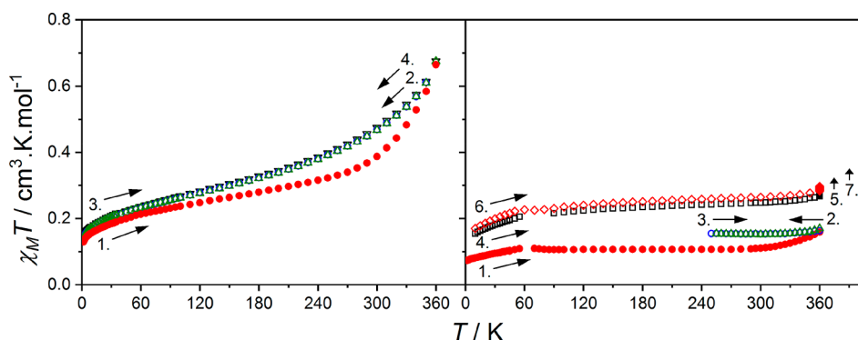
Figure 3. (left) Plot of \chi_M T vs T for solid-state 1(PF 6 )·1.2tol on first heating 1.8–360 K (red ●), first cooling 360–2 K (blue ○), second heating 2–360 K (green △), and second cooling 360–1.8 K (black ▽). (right) Plot of \chi_M T vs T for solid state 1(BPh 4 ) on first heating 1.9–360 K (red ●), first cooling 360–250 K (blue ○), second heating 250–360 K (green △), third heating 10–360 K (□), first holding at 360 K for several hours (■), fourth heating 10–360 K (red ◇), and second holding at 360 K for several hours (red ◆). Numbered arrows indicate the order of the measurements.
