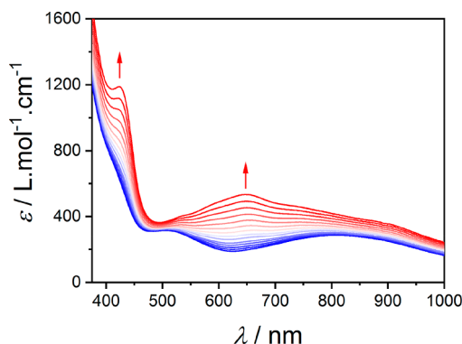
Figure 5. Temperature dependence of the UV–visible spectrum of \mathbf{1}^+ in MeCN from 283 K (blue) to 348 K (red) in 5 K intervals.
