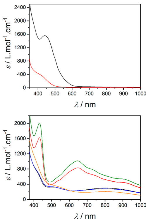
Figure 4. Room-temperature UV–visible spectra of (top) \mathbf{1} (black) and \mathbf{1}\text{-Zn} (red) in DMF and (bottom) \mathbf{1}^+ in MeCN (black), acetone (blue), DMF (orange), DCE (red), and DCM (green).
