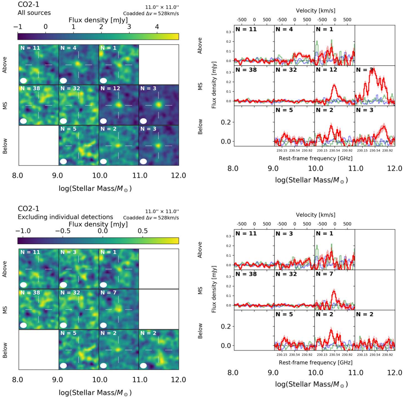
Figure 4. Resulting stacked 2D images (left) and 1D spectra (right) in the bins of SSFRs (above, on, and below the galaxy MS, as discussed in Section 3.2; y-axis) and stellar masses (x-axis). The upper and lower two panels show the results of including and excluding the individually reported direct CO(2-1) detections, respectively (Aravena et al. 2019; Boogaard et al. 2019). The 2D images are coadded between 230.335 \leq \nu_{\text{rest}}/\text{GHz} \leq 230.741 ( \Delta\nu = 528 \text{ km s}^{-1} ) and the white ellipses indicate the mean of the beam size. The 1D spectrum is extracted from the central spaxel (the red solid line). Spectra extracted with random redshifts in place of the MUSE position and with random positions at the correct MUSE redshift are shown by the light blue and green lines, respectively (Section 3.1).
