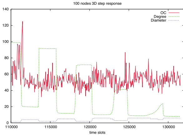
figure 7: Step response in a simulation with 100 Nodes in a 3D configuration (PDOR, schedule length 32 slots)
