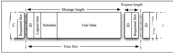
figure 2: Format of the data packet and the time slot
