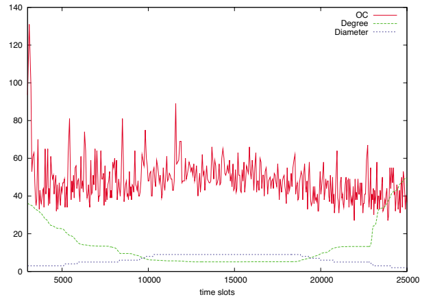
figure 8: Omnicast performance for 64 Nodes in a 2D configuration with slowly varying density (PDOR, schedule length 16 slots)
