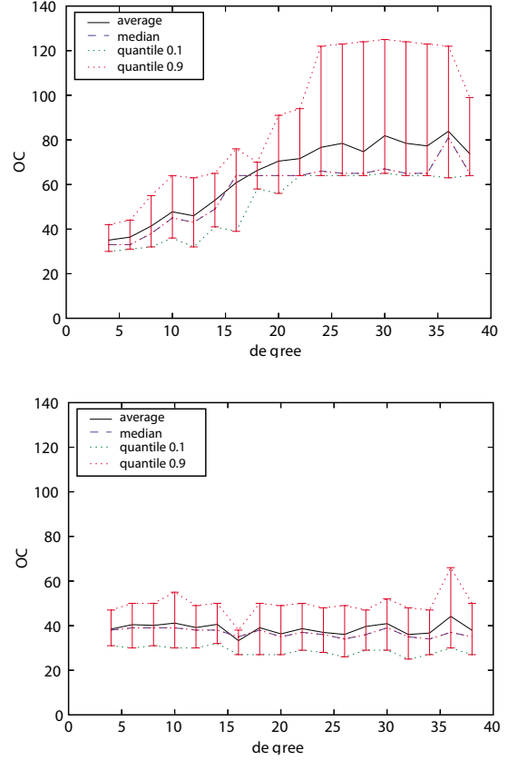
figure 5: Plot of Omnicast performance over graph degree, with 40 nodes, for DDOR (upper: schedule length 64 slots) and PDOR (lower: schedule length 16 slots).
