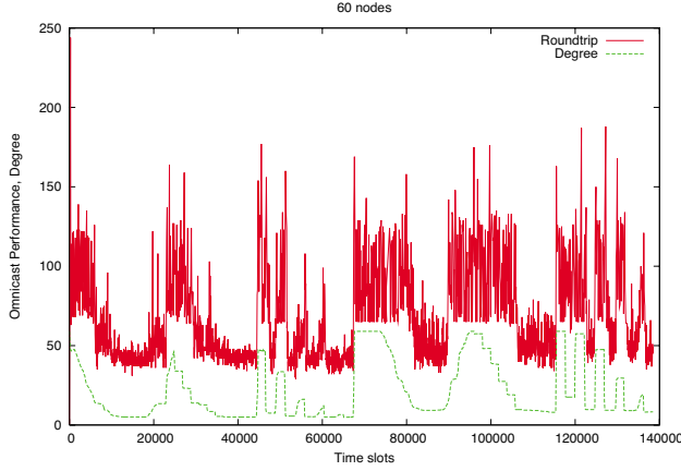
figure 4: A complete simulation run of DDOR with 60 Nodes.
