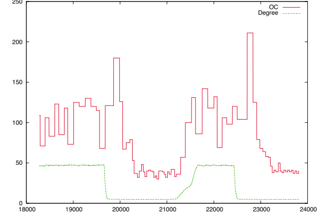
figure 6: Step response in a simulation with 60 Nodes (DDOR)
