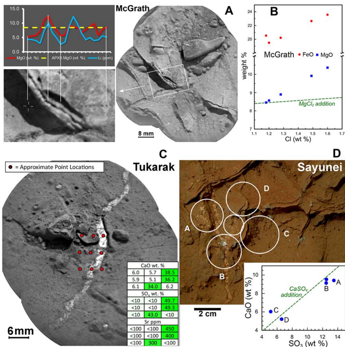
Fig. 5. Geochemical constraints on diagenetic features within the Yellowknife Bay formation.
