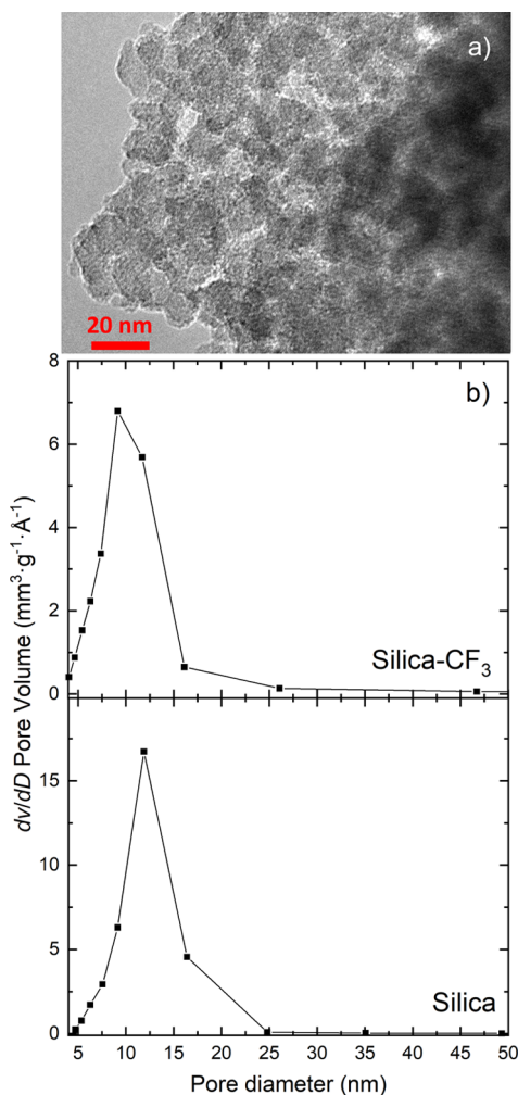
Figure 3. (a) TEM micrograph of Silica and (b) pore size distribution of Silica and Silica-CF 3 .
