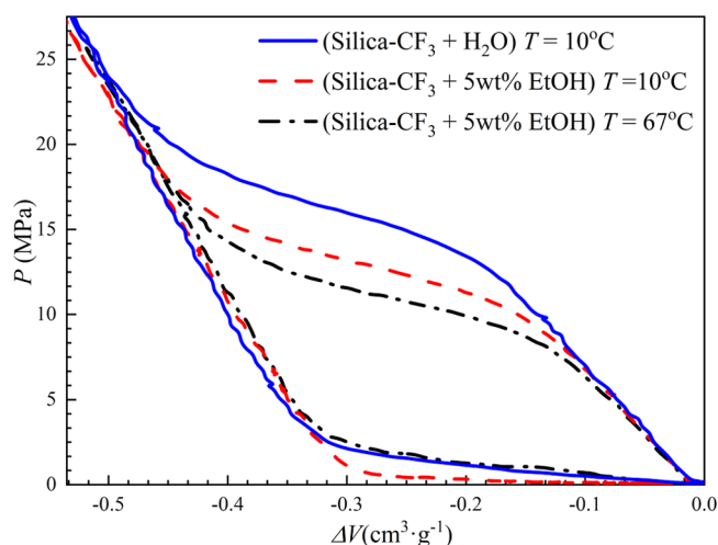
Figure 5. PV isotherms of (Silica-CF 3 + H 2 O/5 wt % EtOH solution) systems at T = 10 or 67 °C at a cycling rate of 200 \text{ MPa}\cdot\text{s}^{-1} .
