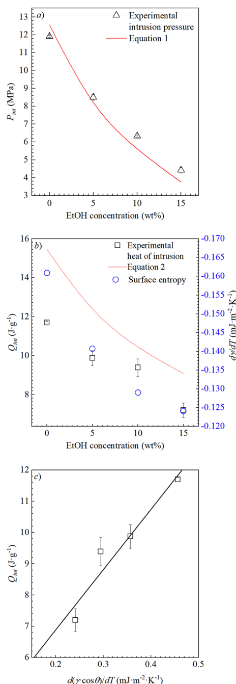
Figure 6. (a) Intrusion pressure, P_{inv} (b) heat of intrusion, Q_{inv} and (c) correlation between the heat of intrusion and surface entropy (black line).
