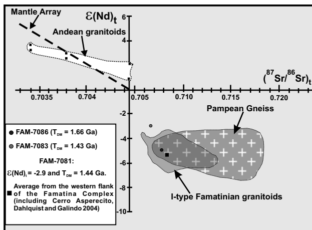
FIGURE 5 | \epsilon\text{Nd}_t vs. initial ^{87}\text{Sr}/^{86}\text{Sr} diagram for Andean (black squares) and Famatinian granitoids. Data from Pankhurst et al. (1998), Pankhurst et al. (2000), Dahlquist and Galindo (2004), and dated igneous rocks in this study. FAM-7081 rhyolite has an anomalously low initial ^{87}\text{Sr}/^{86}\text{Sr} of 0.7000 which suggests post-crystallization modification of its Rb-Sr system.
