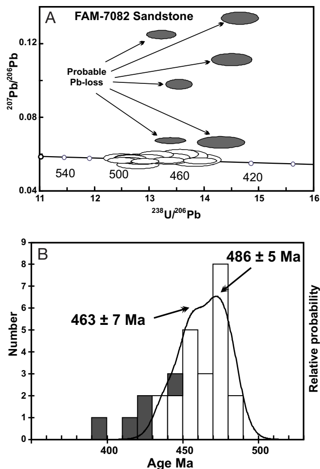
FIGURE 6 | U–Pb detrital zircon ages for FAM-7082 sandstone. A) Tera-Wasserburg plot for grains <500 Ma (see Rapela et al. 2007 for consideration of the older provenance of this sample). Error ellipses are shown at 86.3% confidence limits; individual ages are generally \pm \sim 10 Ma. Those shown in grey plot well above the Concordia, almost certainly indicating Pb-loss in their history, and these data are ignored. The remaining data yield ellipses that fall on the Concordia within error. A few scatter at the younger end of \sim 450 – 460 Ma and may also have suffered the effects of some Pb-loss, but the majorities are densely packed in the interval 460 – 490 Ma. B) The relative probability curve indicates a major peak at 486 \pm 5 Ma with a younger shoulder at 463 \pm 7 Ma (ages estimated by the Sambridge and Compston, 1994, unmixing algorithm). These fall within the known age range of Famatinian magmatism.
