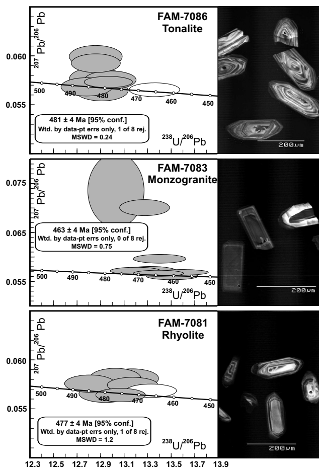
FIGURE 4 | Tera–Wasserburg diagrams for U–Pb SHRIMP zircon analyses of the studied samples (data uncorrected for common-Pb). Ellipses represent 68.7 % confidence limits for each measurement, open ellipses are for points ignored as having been affected by Pb-loss. Age estimates are given for each sample (weighted mean ^{238}U – ^{206}Pb ages).
