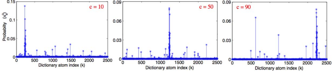
Figure 2. Dictionary atom usage for the data representation of three classes of Caltech-101 [6]: For classes 10, 50 and 90, the Bernoulli distribution parameters \pi_k^c are plotted against the indices of the arranged dictionary atoms. A larger \pi_k^c indicates a more frequent use of the atom in data representation. Due to the discriminative nature of the dictionary, distinct clusters of popular atoms appear. Due to sharing of the atoms by different classes, non-zero values also appear far from the main clusters. The shown relationships between the atoms and the class labels are learned adaptively by our approach.
