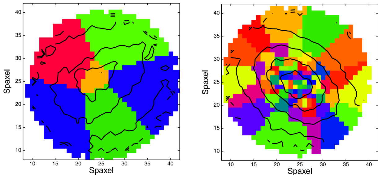
Figure 8. Examples of the binning required to obtain a minimum continuum S/N ratio of 5 per Å (accounting for covariance; for details see Allen et al. 2015; Sharp et al. 2015). Each colour region is one bin. We show a low redshift, low mass ( z = 0.015 , M_* = 10^{8.59} M_\odot ) galaxy (left) and a high-redshift, high-mass ( z = 0.056 , M_* = 10^{10.15} M_\odot ) galaxy (right). SAMI data cubes are re-gridded on to 0.5 arcsec output square spaxels (see Allen et al. 2015; Sharp et al. 2015, for details). Continuum flux is shown by the contours.
