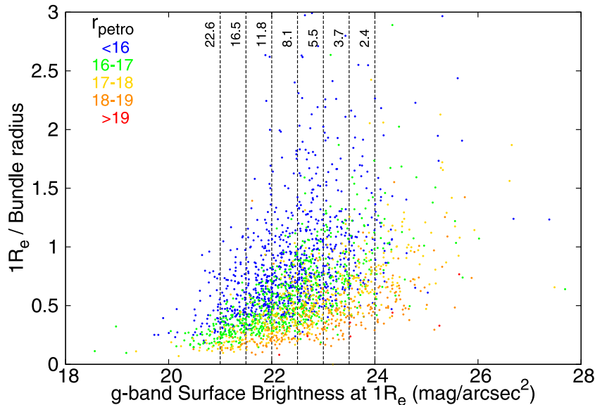
Figure 7. Surface brightness in the g band at 1R_e versus 1R_e as a fraction of bundle radius. Points are colour coded by the Petrosian r magnitude. Vertical dashed lines list the continuum S/N per Å per hexabundle including fill fraction (not per fibre core, which would be a factor of 0.75 higher), expected to be achieved with 3.5 h of integration time for the given surface brightness, based on the B -band SAMI exposure time calculator. The galaxies with lowest surface brightness at 1R_e tend to be larger, and therefore can be binned to increase S/N.
