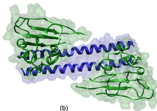
Figure 1 Overall structure of PfNapS. (a) Domain diagram for NAP/SET crystal structures determined so far. Architecture of PfNapS, yNAP-1, Vps75, hSET and PfNapL highlighting the 'accessory domain' in yNAP-1 (coloured yellow) which is missing in the remaining 4 structures (set to scale). (b) Structure of the PfNapS dimer. Each monomer of PfNapS contains domain I comprised of dimerization helix \alpha 2 and domain II comprised of a \beta sub-domain (4 anti-parallel \beta strands) and \alpha -helices.
