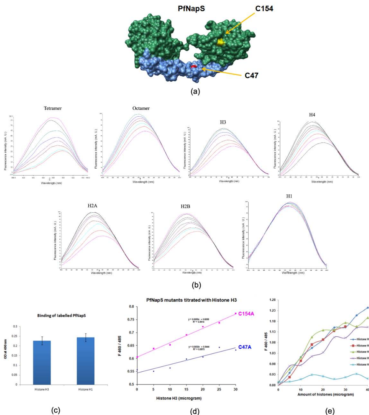
Figure 4 PfNapS-histone interaction studies using fluorescence spectroscopy (a) PfNapS dimer is shown as molecular surface. Domains I and II are coloured blue and green respectively. The residues Cys47 and Cys154 are coloured red and yellow and are indicated. (b) Fluorescence emission spectra of PfNapS in presence of increasing concentrations of histones. A hypsochromic shift (blue shift) was observed on binding of histones. However in case of histone H1 no such change was observed. Fluorescence intensity was measured after incubating 75 micro gram of PfNapS protein with 5, 10, 15, 20, 25, 30, 35, 40, 45, and 50 micrograms of histones. All experiments were repeated thrice. (c) Effect of labeling on binding of PfNapS to histones H3 and H1. (d) Graph representing hypsochromic shift (F460/485) in fluorescence of two PfNapS mutants as a function of amount of H3 histone. (e) Graph representing differential binding of linker histone H1 with respect to core histones. There is no shift in fluorescence on binding of H1, however, core histones show hypsochromic shift (F460/485) in fluorescence.
