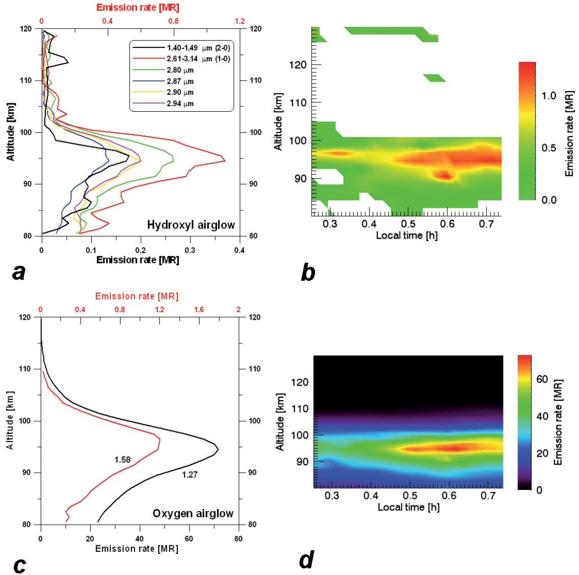
Fig. 2. Limb vertical profiles of the O_2 and OH nightglow emissions versus tangent altitude. Panel a ): vertical profiles of the OH emission at 2.80\ \mu\text{m} (green), 2.87\ \mu\text{m} (blue), 2.90\ \mu\text{m} (yellow), 2.94\ \mu\text{m} (magenta), plus all of these integrated from 2.61 to 3.14\ \mu\text{m} (shown in red, only this one corresponding to the x axis on top in the same color, all the others refer to the bottom axis) and from 1.40 to 1.49\ \mu\text{m} (black). Panel b ): the local distribution of the integrated bands (red curve of panel a ) versus local time and tangent altitude of the closest point of the tangent limb to the planet. It can be seen that the distribution of the OH emission varies even within a single orbit. For comparison, the O_2 emission at 1.27 (black, bottom axis) and 1.58\ \mu\text{m} (red, upper axis) is shown for the same orbit in panel c ), and its variability in panel d ). In all cases the instantaneous geometrical vertical resolution from the distance of 10\,800\ \text{km} to 13\,700 is better than 3.5\ \text{km} . In order to improve the signal to noise ratio, pixels are averaged over the latitude range 10 – 35^\circ\ \text{N} and all profiles are smoothed with a step of 2\ \text{km} in height.
