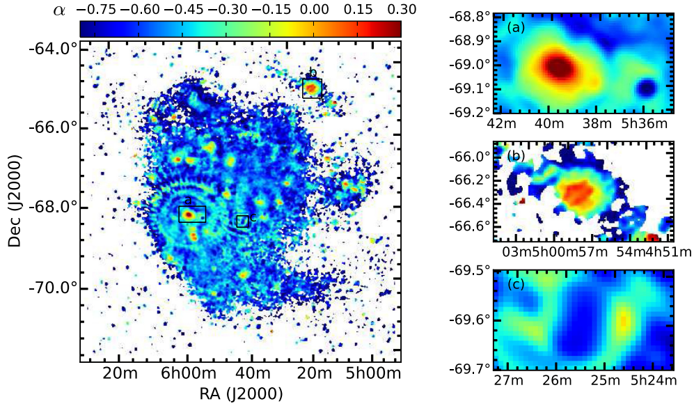
Figure 6. Spectral index map of the LMC calculated from the GLEAM 166 MHz and the 1.4 GHz images. Panels (a) and (b) on the right show HII regions: 30 Doradus and N11. Both have positive \alpha indicating the emission is dominated by thermal emission. At the right corner of panel (a) also shows a prominent source, the supernova remnant 1987A, which has a steep negative \alpha indicating the emission is dominated by non-thermal synchrotron emission. Panel (c) shows supernova remnant N132D. It has a similar \alpha as the supernova remnant 1987A.
