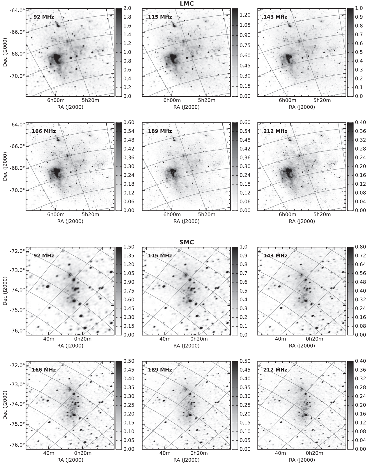
Figure 1. Selected radio images of the LMC and SMC from the GLEAM survey. From top left to bottom right are images centred at 92, 115, 143, 166, 189, and 212 MHz. The grey scale is in units of \text{Jy beam}^{-1} .
