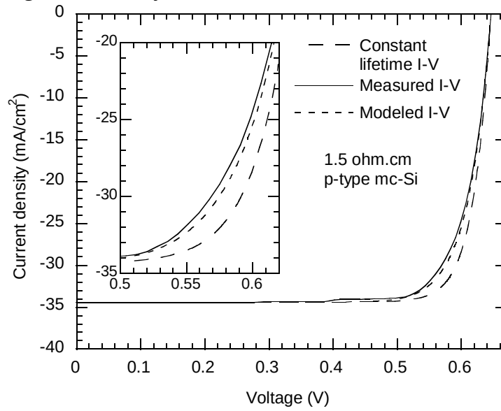
Figure 5: Implied and measured one-sun I-V curves for the 1.5 \Omega .cm cell. The inset shows a magnified version of the maximum-power region. The constant lifetime I-V curve is for a cell with no injection-level dependence below open-circuit, resulting in a higher fill factor.
