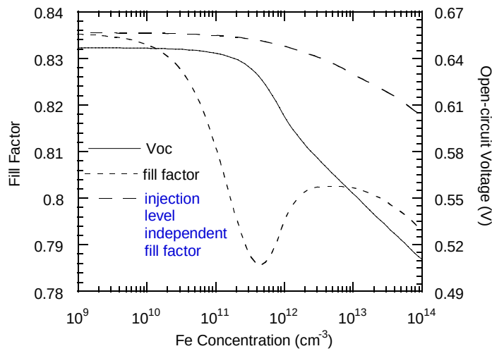
Figure 6: Effect of Fe_i concentration on V_{OC} and fill factor as modeled for a 1.5 \Omega .cm cell of thickness 0.03cm and with J_{0e}=3\times 10^{-13} A/cm 2 . Also shown is the fill factor curve for a recombination centre that has an injection-level independent bulk lifetime.
