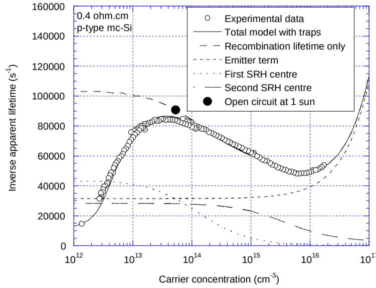
Figure 2: Inverse apparent lifetime versus carrier concentration for a 0.4 \Omega .cm mc-Si cell precursor. The two SRH curves and the emitter term are shown separately. The solid circle represents open-circuit conditions under one-sun illumination.
