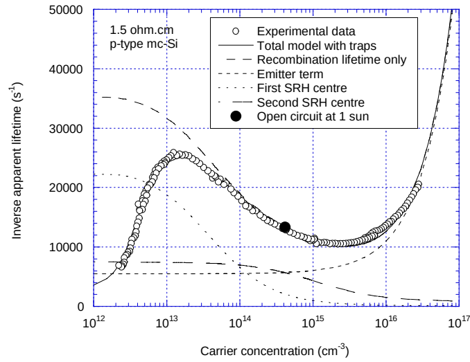
Figure 1: Inverse apparent lifetime versus carrier concentration for a 1.5Ω.cm mc-Si cell precursor. As well as showing the total injection-level dependent model, the constituent parts, namely the two SRH centres and the emitter term, are also shown. The solid circle represents open-circuit conditions under one-sun illumination.
