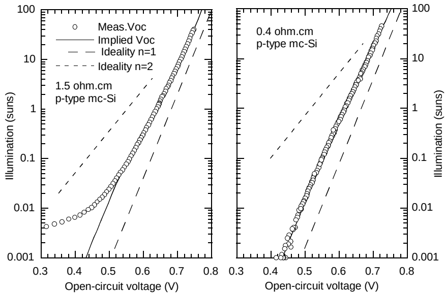
Figure 3: Implied and measured illumination- V_{OC} curves for both the 1.5 \Omega .cm and 0.4 \Omega .cm cells. Lines representing idealities of 1 and 2 are included. The effect of a shunt resistance is evident for the 1.5 \Omega .cm cell at low voltages.
