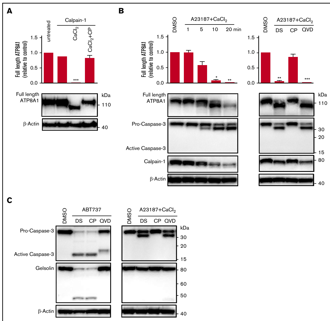
Figure 3. ATP8A1 is a direct substrate of calpain. (A) Mouse platelet membrane fractions (10 \mu g) remained untreated or were incubated with purified human calpain-1 (4U) in the absence or presence of CaCl 2 (5 mM) or CP (50 \mu g/mL) at room temperature for 30 minutes. Samples were then denatured for western blot analysis of ATP8A1 and \beta -actin. (B-C) Washed mouse platelets ( 5 \times 10^7 ) were treated with vehicle (DMSO) or A23187 (1 \mu M; room temperature) in the presence of CaCl 2 (2 mM) for the indicated time. In some experiments, platelets were preincubated with DMSO (DS), CP (50 \mu g/mL) or QVD (25 \mu M) at room temperature for 15 minutes before treatment with A23187 (20 minutes) or ABT737 (1 \mu M, 37°C, 2 hours, in the absence of CaCl 2 ). Platelets were subsequently lysed for western blot analysis of ATP8A1, Caspase-3, Calpain-1, Gelsolin, and \beta -actin. Immunoblots are representative of n = 3 independent experiments. Bar graphs represent blot quantification of full-length ATP8A1 by densitometric analysis (means \pm SEM, n = 3 ) of stained bands using Image J, corrected for loading control ( \beta -Actin). Statistical significance was calculated using Student 2-tailed t test. * P < .05 ; ** P < .01 ; *** P < .001 .
