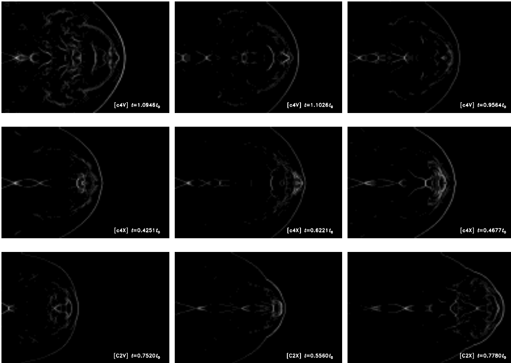
Fig. 16. Plots of |\nabla p| , delineating the presence of shocks. Panel dimensions are the same as in Figures 10-15.
