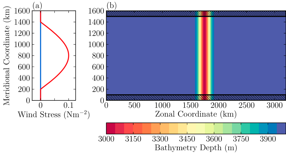
FIG. 1. (a) The meridional wind stress profile ( \text{N m}^{-2} ) and (b) the physical domain. Colors indicate domain depth (m). Shading shows the location of the sponge regions in the buoyancy-forced simulations.
