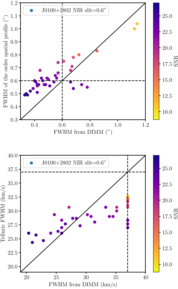
Figure 6. Same as Fig. 5 but for the NIR frames of SDSSJ0100+2802, observed with a slit = 0.6 arcsec.
