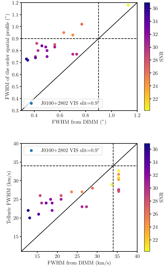
Figure 5. FWHM of the spectral order spatial profiles (upper panel) and average FWHM of the telluric model (lower panel) as a function of the FWHM at \sim 950 \text{ nm} of the seeing disc for the VIS frames of the literature quasar SDSSJ0100+2802, which was observed with a slit = 0.9 \text{ arcsec} . The dots are coloured according to the SNR of the corresponding frame (see the scale in the sidebar). The dashed lines indicate the slit value.
