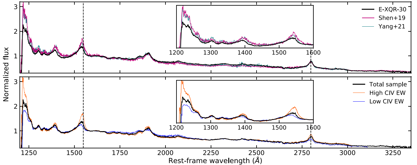
Figure 9. Upper panel: composite spectrum of the total E-XQR-30 sample rebinned to 250 \text{ km s}^{-1} (black curve), compared with composite spectra of z \simeq 5.7 - 7 quasars from Shen et al. (2019) and Yang et al. (2021). Bottom panel: composite E-XQR-30 spectrum for quasars with high (low) equivalent width of the C IV line, as shown by the orange (blue) curve, compared with the total E-XQR-30 composite spectrum. Vertical lines indicate the rest-frame wavelength of C IV and Mg II emission lines considering z_{\text{MgII}} (Table 1). Insets show a zoom-in on the spectral region between Ly \alpha and C IV.
