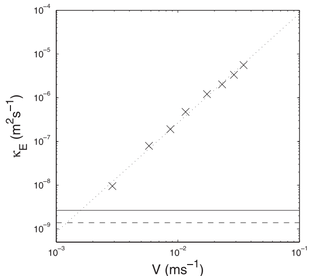
FIG. 2. Plot of \kappa_E as a function of \bar{V} : the solid line is the calibrated value of \kappa_E for \bar{V} = 0 (i.e., no rod stirring), and the dashed line shows the accepted value for molecular diffusion of salt in water, \kappa_m = 1.39 \times 10^{-9} \text{ m}^2 \text{ s}^{-1} (Washburn 2003). The least squares fit, shown by the dotted line, is that of the relationship \kappa_E = 0.027\bar{V}^{2.5} .
