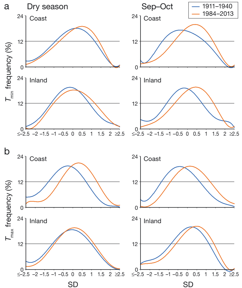
Fig. 6. Curves of best fit for changes in frequency of daily (a) minimum temperature ( T_{\min} ) and (b) maximum temperature ( T_{\max} ) over northern Australia between the coastal and inland stations for the Dry season (left) and the early Build-up (Sep–Oct) (right), between 1911–1940 and 1984–2013, as measured against the 1961–1990 SD values
