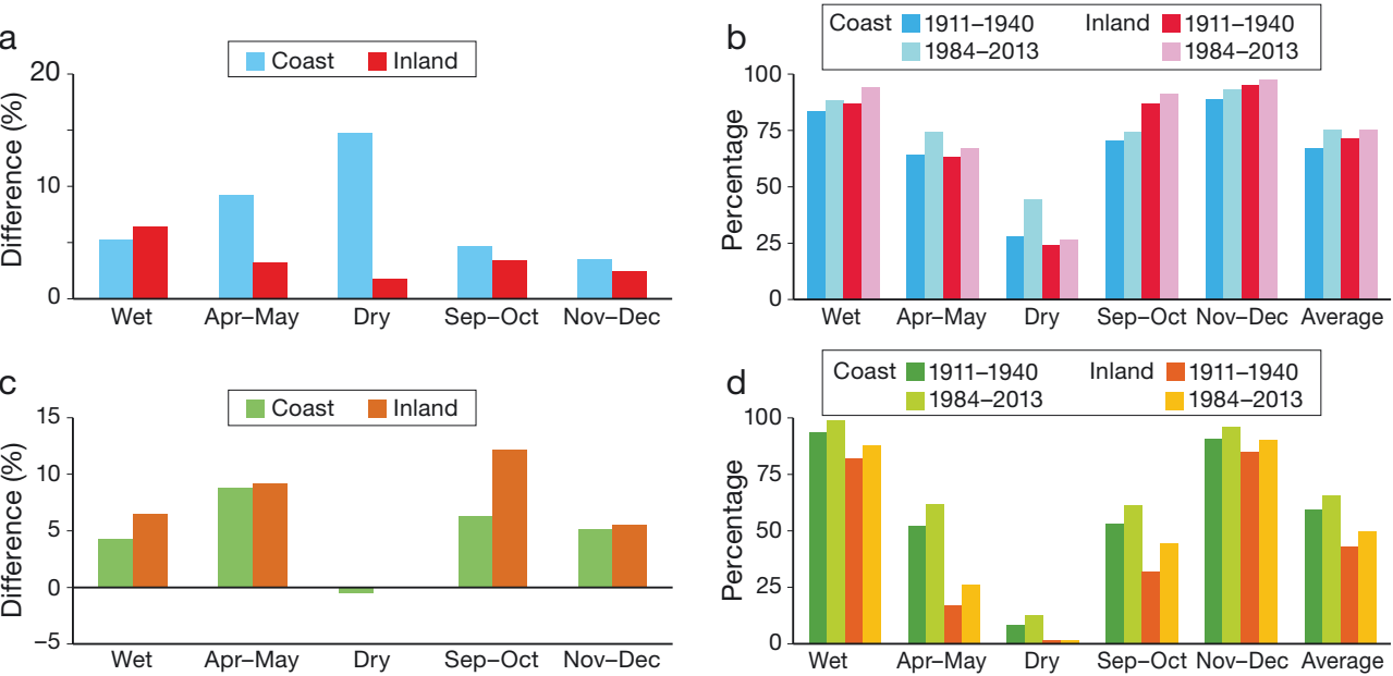
Fig. 5. Percentage change in total days and in overall percent of days (a,b) >30^{\circ}\text{C} and nights (c,d) >21^{\circ}\text{C} for coastal and inland locations between 1984–2013 and 1911–1940
