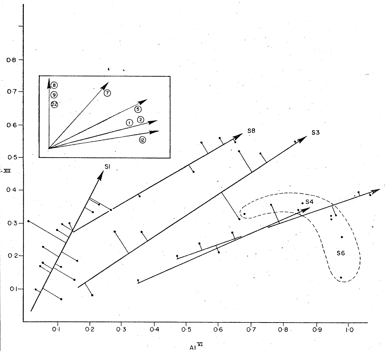
Fig. 9. Trends of \text{Na}^{\text{X-XII}} versus \text{Al}^{\text{VI}} in zoned amphiboles from quartz-free rocks and S8 which contains only a few percent quartz.
