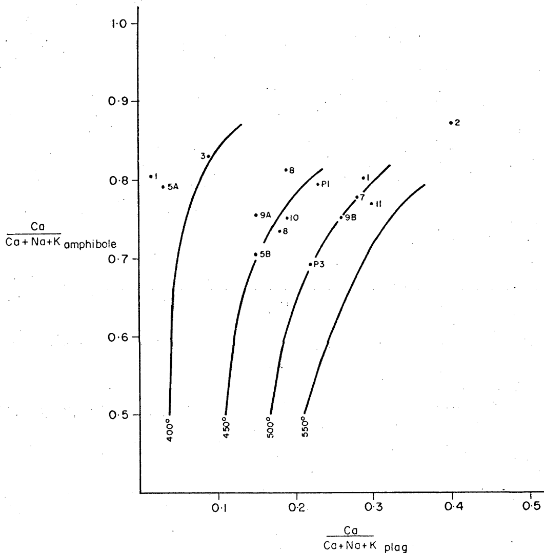
Fig.14. Distribution of \text{Ca}/(\text{Ca}+\text{Na}+\text{K}) between plagioclase and Ca amphibole. Isotherms after Perchuk (1966). Note the poor temperature agreement between the pairs 5A, 5B and 9A, 9B. Amphibole-plagioclase pairs are from adjacent grains and less than 20 microns apart.
