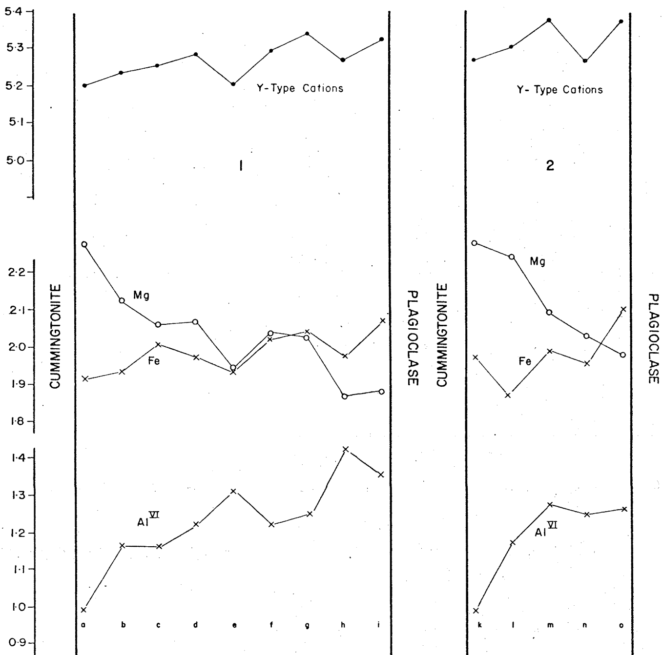
Fig. 12. P2B: Zoning of 2 hornblende rims from boundary with cummingtonite to boundary with plagioclase. Note that although Mg increases towards cummingtonite boundary, the total number of Y type cations appears to decrease slightly.
