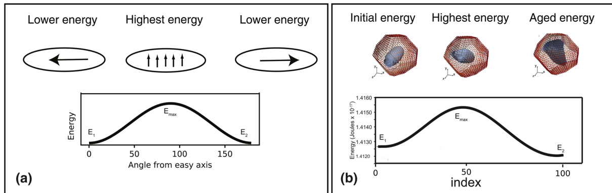
Figure 15. Energy barriers to magnetization switching from one easy axis to the other. (a) Néel particle (uniaxial SD). (b) Single vortex particle with multiple easy axes. SD, Single Domain.
