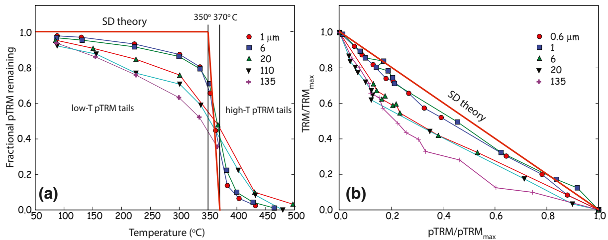
Figure 2. (a) Stepwise thermal demagnetization of pTRMs imparted by applying a small DC field during cooling from 370 to 350°C in magnetite of known grain size. Between 50% and 90% of the remanence unblocks below (a low temperature pTRM tail) or above (a high temperature pTRM tail) the pTRM blocking temperature range. Failure of reciprocity is most extreme for the largest grain sizes. (b) Arai plots for paleointensity experiments on the synthetic specimens shown in (a). Note that the X-axis is somewhat unusual in that the pTRM was normalized by the maximum pTRM acquired (total TRM) and not the initial TRM as is the usual practice. [Data of Dunlop and Özdemir (2001); figure modified from Tauxe et al. (2010)].
