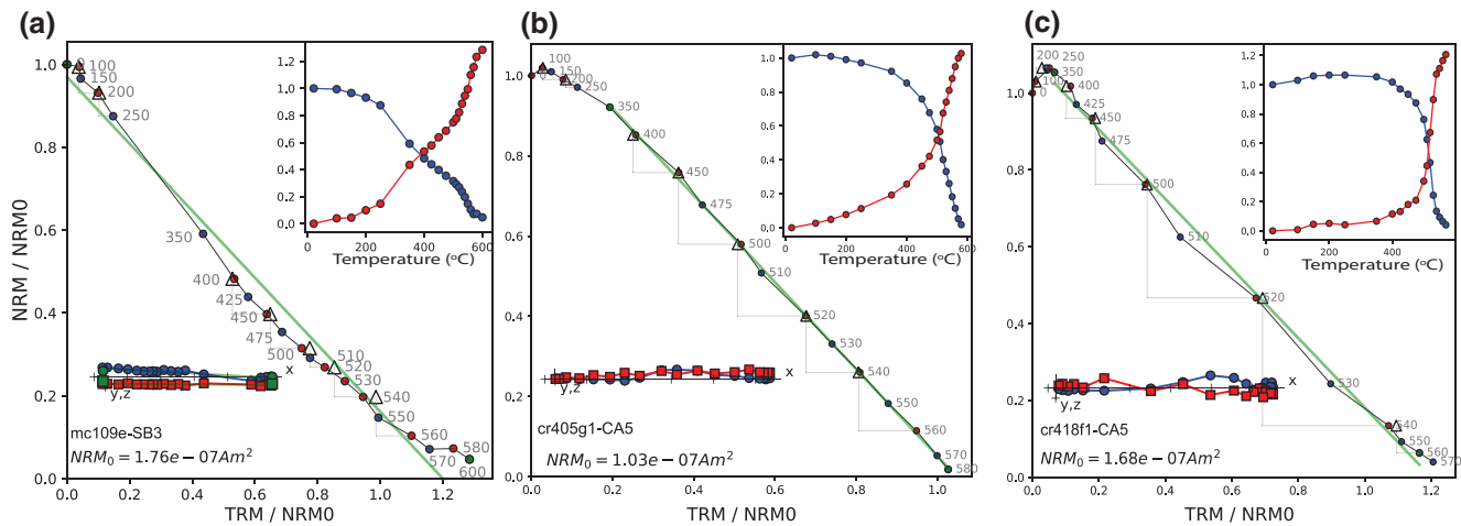
Figure 12. Unusual behavior during the IZZI experiment. Arai plots with best-fit line in green. ZI (IZ) steps are plotted as blue (red) circles; pTRM check steps are plotted as triangles. Lower left insets: Zijderveld (1967) diagrams of remanence decay. X-Y (X-Z) projection plotted as blue circles (red squares). Upper right insets: remanence decay (acquisition) plotted as blue (red) symbols. (a) Specimen altered during the experiment. (b)-(c) Specimens acquired a VRM during aging in a 70 \mu T field antiparallel to the NRM. The plots were made with thellier_gui.py in the PmagPy software package of Tauxe et al. (2016). IZ, zero-field; pTRM, partial thermal remanent magnetizations; ZI, in-field.
