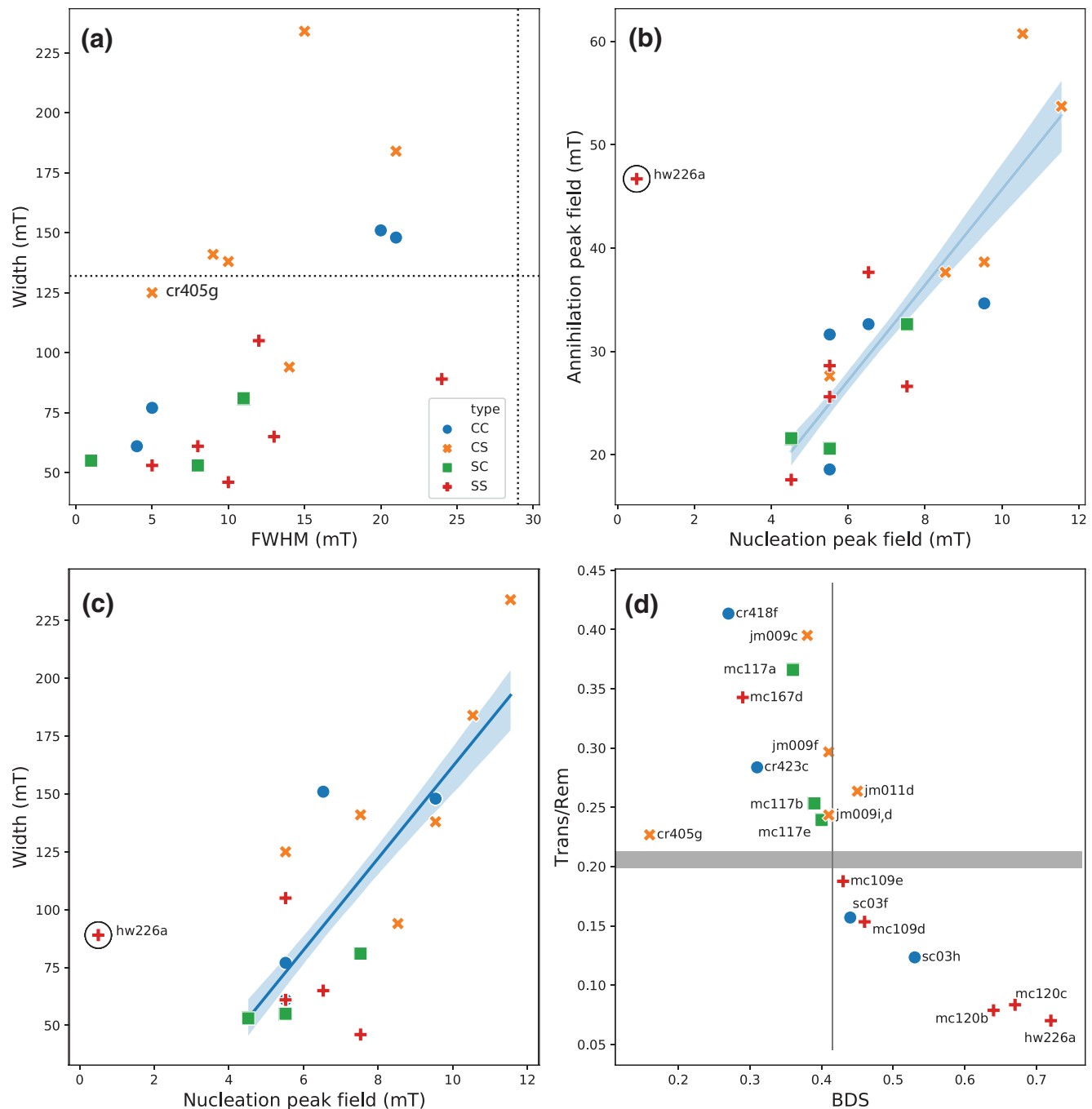
Figure 11. (a) “Carvallo plot” (Carvallo et al., 2006) with width of the FORC distribution along the B_i axis plotted against the full-width half-maximum (FWHM) of a vertical profile through the peak of the coercivity distribution. Threshold values recommended by Carvallo et al. (2006) for FWHM and width are 29 mT and 132 mT, respectively. (b) Annihilation peak field (APF) versus nucleation peak field (NPF). (c) Width versus nucleation peak field (NPF). Best-fit line with bootstrap uncertainty bounds were calculated without including data for specimen hw226a. (d) Transience to remanence ratio (T/R in Table 2) plotted against bulk domain stability (BDS). All values are listed in Table 2.
