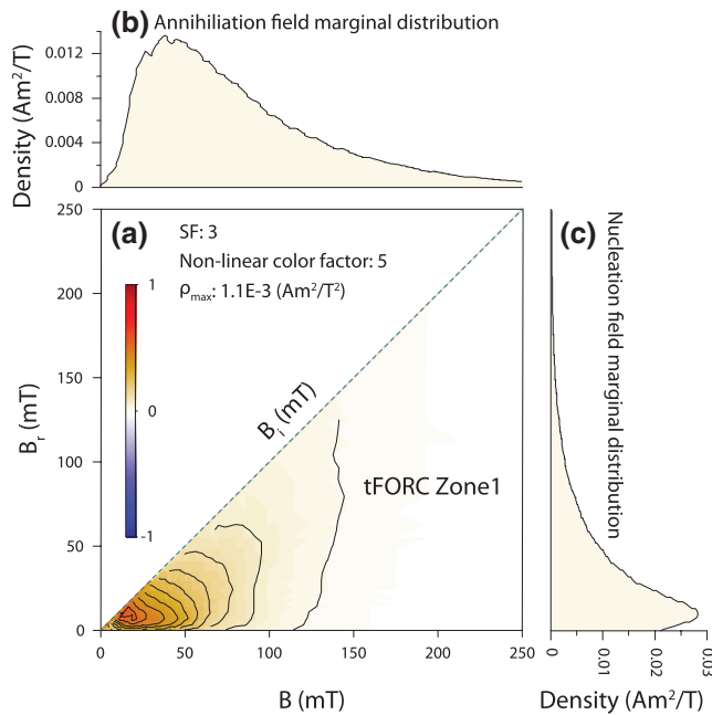
Figure 8. Example of the marginal distribution of nucleation and annihilation fields from Zone 1 of the tFORC distribution. (a) Zone 1 of the tFORC distribution for sample jm011d. (b) and (c) Marginal distributions of the annihilation and nucleation fields, respectively. The smoothing factor (SF) and nonlinear color scale for the FORC diagram are specified in the inset. FORC, first-order reversal curve; tFORC, transient FORC.
