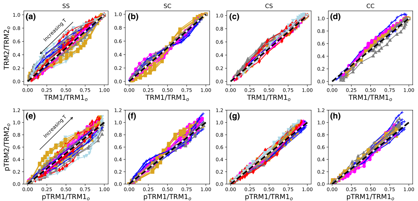
Figure 14. Comparison of (un)blocking temperature spectra between fresh and aged specimens. The curves for demagnetization and remagnetization for the experiments are shown in Figures S2 and S3. The expected line of equal (un)blocking at a given step is shown by the black dashed line in each plot. (a–d) TRM unblocking (zero field steps). X-axis is magnetization remaining at each temperature step for the fresh TRM (TRM1); Y-axis is magnetization remaining for each aged specimen at the same temperature step (TRM2). The initial TRM is at the upper right-hand corner of the plot. (e–h) TRM blocking (infield steps). X-axis is magnetization acquired at each temperature step of the fresh pTRM (pTRM1); Y-axis is magnetization acquired for each aged specimen at the same temperature step (pTRM2). The final pTRM is at the upper right-hand side of the plot. (a, e) SS group specimens. (b, f) SC group specimens. (c, g) CS group specimens. (d, h) CC group specimens. pTRM, partial TRM; TRM, thermal remanent magnetizations.
