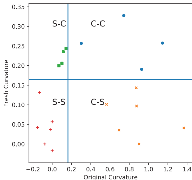
Figure 6. Comparison of curvature as quantified by \tilde{k} for the fresh TRMs of Santos and Tauxe (2019) versus original TRMs (see Table 1 for references). Specimens from samples with low curvature (S) either remained straight (SS) or became significantly curved (SC) after being given a fresh TRM. Specimens from samples with high curvature (C) either became straight (CS) or remained curved (CC) after being given a fresh TRM. All CC specimens have significantly less curved Arai plots than in the original experiments, so they have “fragile” curvature.
