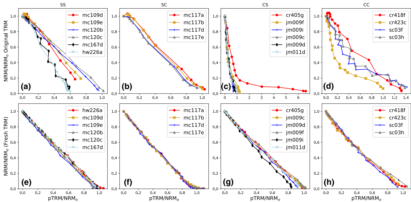
Figure 5. Arai plots for specimens from Santos and Tauxe (2019) and references therein. (a, e) SS behavior; (b, f) SC behavior; (c, g) CS behavior; and (d, h) CC behavior. Top row: Arai plots from the original studies. Bottom row: same as top row, but for the fresh TRM experiments of Santos and Tauxe (2019). Values for curvature are listed in Table 2. TRM, thermal remanent magnetizations.
