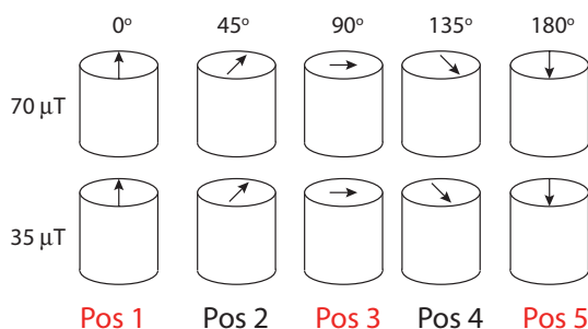
Figure 9. Design of the aging experiment. Sister specimens for each sample from Santos and Tauxe (2019) were given a fresh TRM along the direction of the arrows in a laboratory field of 70 \mu T . Specimens were placed in one of five positions (Pos 1–Pos 5) in either a 70 \mu T or 35 \mu T field.
