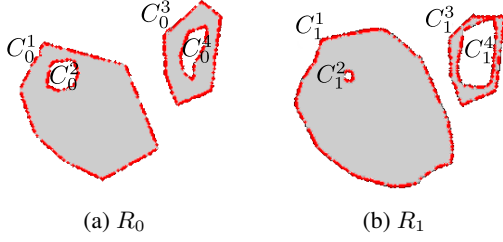
Figure 2: Depicted is region R_t for t = 0 and t = 1 .
