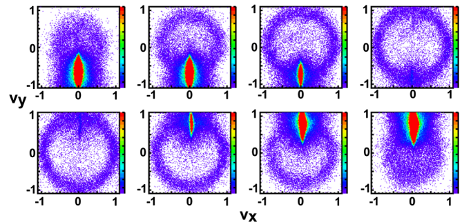
FIG. 21 (color online). Slices in vertical velocity v_z of the spherical shell of atoms in velocity space (in units of v_{\text{rec}} ) for a collision of two BECs. The data are similar to that of Perrin (2007). All plots use the same linear false color scale. The scattering halo is the circular shell which intersects the BECs.
