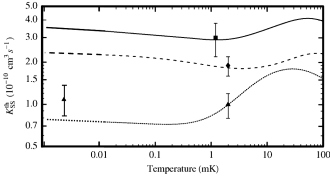
FIG. 10. Experimental Penning ionization loss rate coefficients for an unpolarized gas of helium atoms in the metastable 2^3S_1 state, compared to single-channel theory (McNamara et al. , 2007). Dashed curve: theory for ^3\text{He}-^3\text{He}^* , and experimental point at T = 2 mK (diamond); solid curve: theory for ^4\text{He}-^3\text{He}^* , and experimental point at T = 1 mK (square); dotted curve: theory for ^4\text{He}-^4\text{He}^* , and experimental points at T = 2 mK and T = 3 \mu\text{K} (triangle). The T = 3 \mu\text{K} point is from Partridge et al. (2010), deduced from experiments in an optical dipole trap; see Sec. III.B.2.
