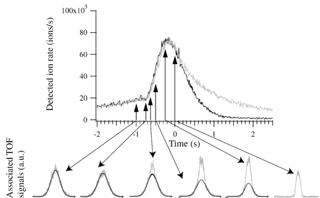
FIG. 24. Ion signal during the last stage of rf evaporation. Its sharp increase at t_{\text{th}} = -0.7 \text{ s} indicates that the cloud crosses the Bose-Einstein threshold. This is confirmed by switching off the trap at various times and measuring the time-of-flight signal. For t > t_{\text{th}} a double structure is clearly visible indicating the presence of a Bose-Einstein condensate. The upper lighter curve corresponds to a situation where the rf shield is always on, whereas it is off after BEC formation for the lower darker curve. The difference indicates that without an rf shield, the condensate heats up rapidly (see text). From Seidelin et al. , 2003.
