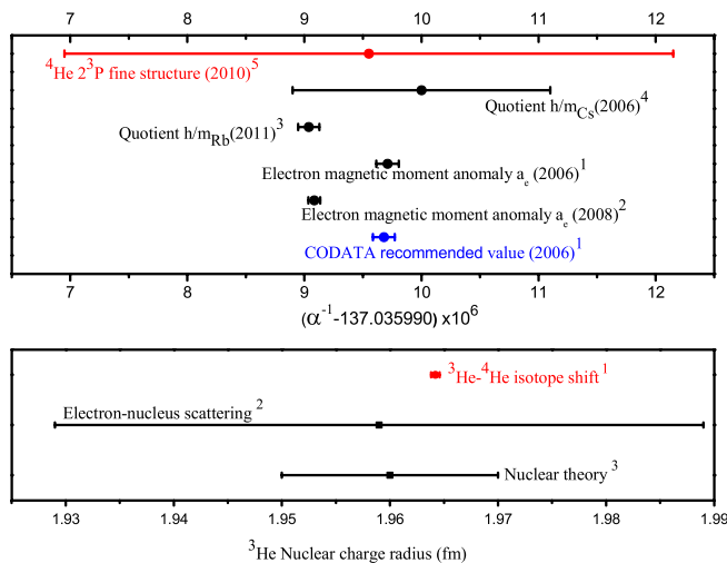
FIG. 15 (color online). Top: Comparison of most updated \alpha determinations [(1) Mohr, Taylor, and Newell, 2008, and references therein; (2) Hanneke, Fogwell, and Gabrielse, 2008; (3) Bouchendira et al. , 2011; (4) Gerginov et al. , 2006] with the recent \alpha value determined by ^4\text{He } 2^3P_0 - 2^3P_2 fine structure [(5) Smiciklas and Shiner, 2010]. Bottom: Comparison of the ^3\text{He} nuclear charge radius measured from the ^3\text{He} - ^4\text{He} isotope shift [(1) Marin et al. , 1995; Morton, Wu, and Drake, 2006b; Shiner, Dixon, and VEDantham, 1995; Zhao, Lawall, and Pipkin, 1991] and by electron-nucleus scattering [(2) Amroun et al. , 1994] and calculated with nuclear theory [(3) Pieper and Wiringa, 2001].
