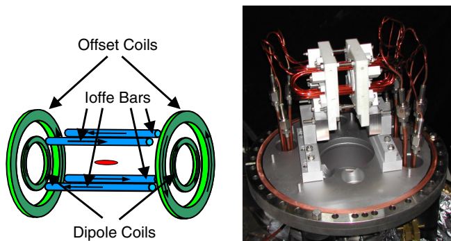
FIG. 5 (color online). Left: Schematic view of a Ioffe-Pritchard trap configuration. Right: Photograph of an actual magnetic trap. The current carrying coils and bars are created from hollow copper tubes mounted on two ceramic plates. Between the plates, the Ioffe bars are visible. The trap coils are water cooled through the hollow copper tubes. The whole assembly has a linear dimension of about 15 cm.
