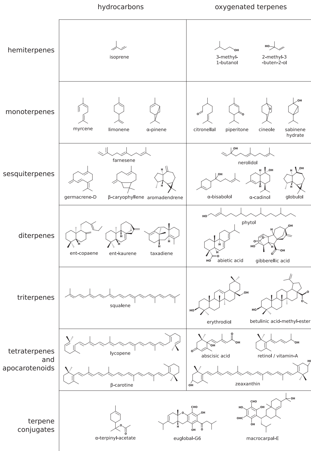
Fig. 1. Representatives of the main classes of terpenes, showing acyclic, monocyclic and polycyclic representatives of both terpene hydrocarbons and oxygenated terpenes.
