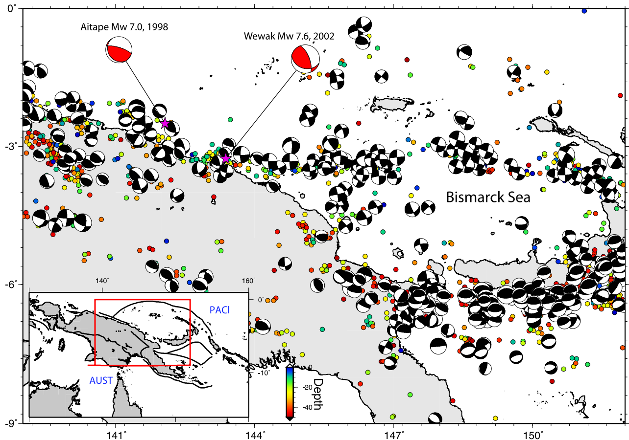
Figure 2. Focal mechanism for earthquakes, from the Global CMT catalogue, with Mw > 5.5 and depth less than 100 km. Seismicity is from ISC Bulletin with magnitudes more than 4.8 and depth between 0 and 60 km depth (1964 to April 2012).
