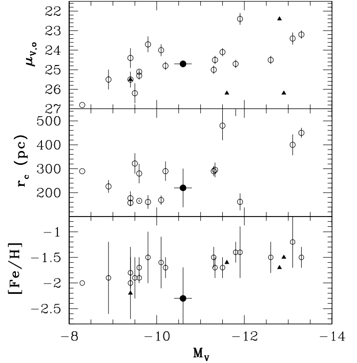
FIG. 9.—Comparison of the structural and chemical properties of the Virgo dSph (filled circle) with measurements for the dwarf spheroidals in the Local and M81 Groups (open circles). The top panel shows central surface brightness, the middle panel shows core radius, and the bottom panel shows metallicity, with the error bars representing the metallicity dispersion. The filled triangles denote measurements of faint dE/dSph galaxies in the Virgo Cluster from Caldwell (2006). The Local Group data come from the compilations of Irwin & Hatzidimitriou (1995), Grebel et al. (2003), and McConnachie & Irwin (2006), with additional information for individual dwarfs from Saviane et al. (1996), Palma et al. (2003), and Harbeck et al. (2005). The M81 dwarf data come from Caldwell et al. (1998). Note that the properties of the Virgo dwarf are completely consistent with those of dwarfs in these low-density systems.
