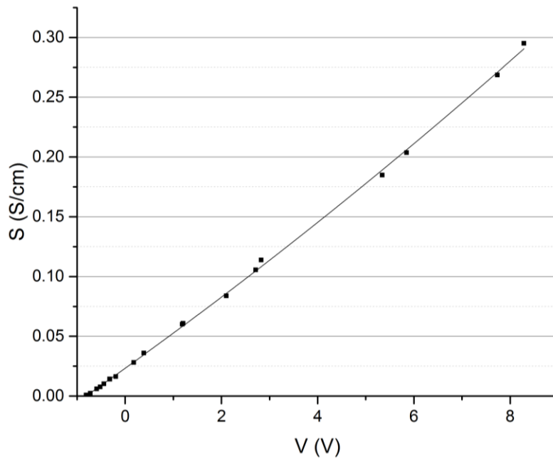
Figure 1. Plot of conductivity against measured voltage in induction coil, with quadratic line of best fit.
