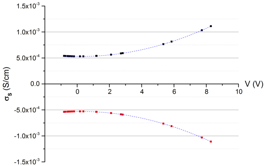
Figure 4. Plot of uncertainty as calculated from (dots) Equation 13 using \sigma_b from Equation 14 and (line) quadratic fit of \sigma_s from Equation 8.
