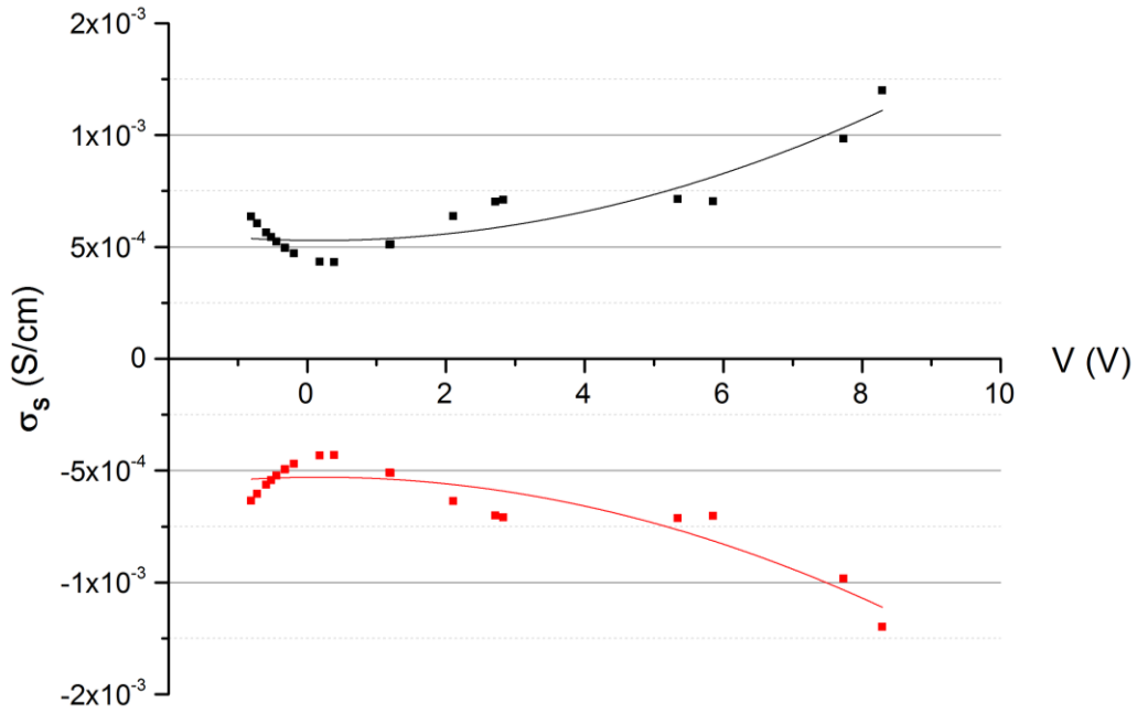
Figure 3. Quadratic fit of uncertainty in conductivity against measured voltage in induction coil.
