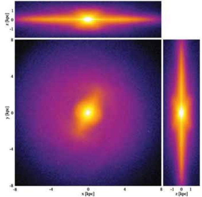
Figure 2. Mass surface density of the model projected onto the x – y , x – z , and y – z planes as indicated. Note the boxy shape and X-structure in the y – z projection at right.
