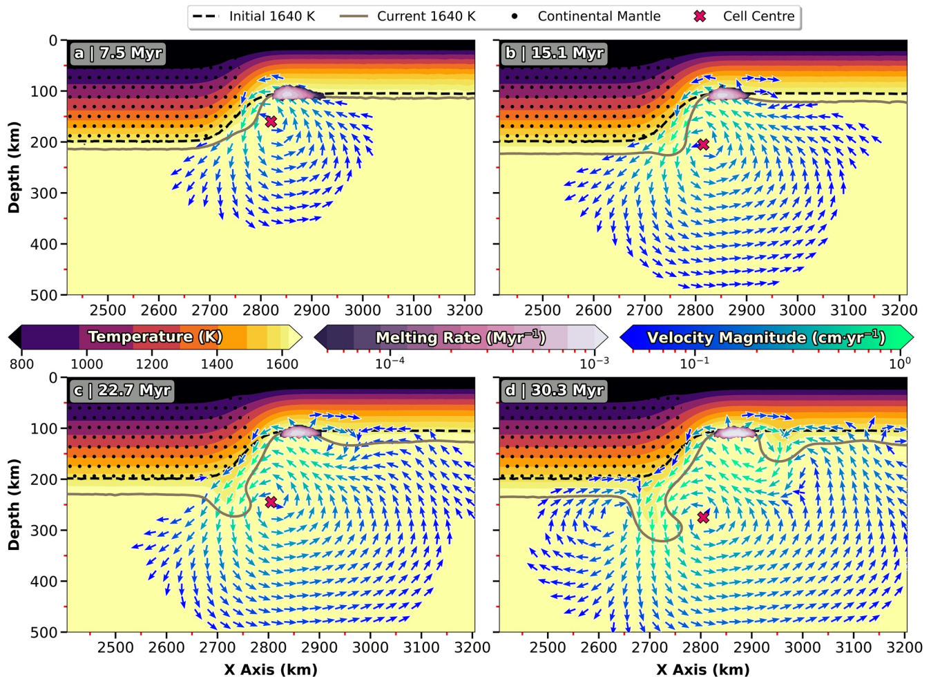
Figure 3. Development of an instability adjacent to the right step of the reference 2-D case. Background colors represent temperature, with the current and initial location of the 1,640 K isotherm, a convenient proxy for downwellings, highlighted by solid gray and dashed black lines, respectively. Black dots depict the location of continental mantle. Arrow glyphs highlight the areas of most intense velocity, where the magnitude is higher than 0.5 \text{ mm yr}^{-1} , as indicated by their color. Areas experiencing melting are represented as a superimposed surface, colored by melting rate. The red cross denotes the center of the cell.
