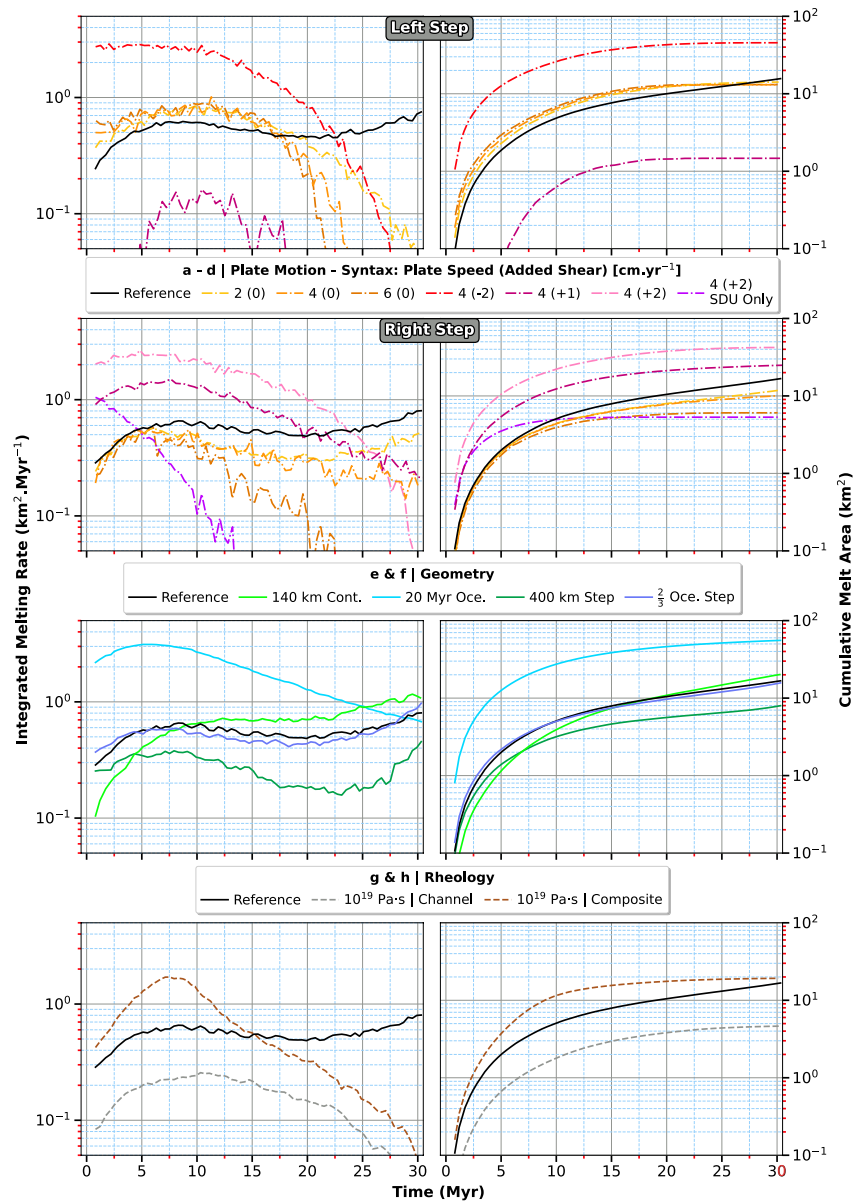
Figure 6. (a), (c), (e), and (g) Integrated melting rate measured at the right step (if not specified), as a function of time. Values correspond to the full integral in space of interpolated melting rates as recorded by particles. (b), (d), (f), and (h) Cumulative melt area, corresponding to the cumulative sum of melting rate additionally integrated in time. (a), (b), (c), and (d) Influence of asthenospheric flow, “Reference” corresponds to an enclosed simulation. (e) and (f) Effect of step geometry, “Reference” corresponds to “40 Myr Oce.”, “200 km Step”, “200 km Cont.”, and a material boundary halfway along the step. (g) and (h) Role of viscosity, “Reference” corresponds to a purely diffusion creep channel-free profile with a minimum viscosity of 10^{19} Pa s.
