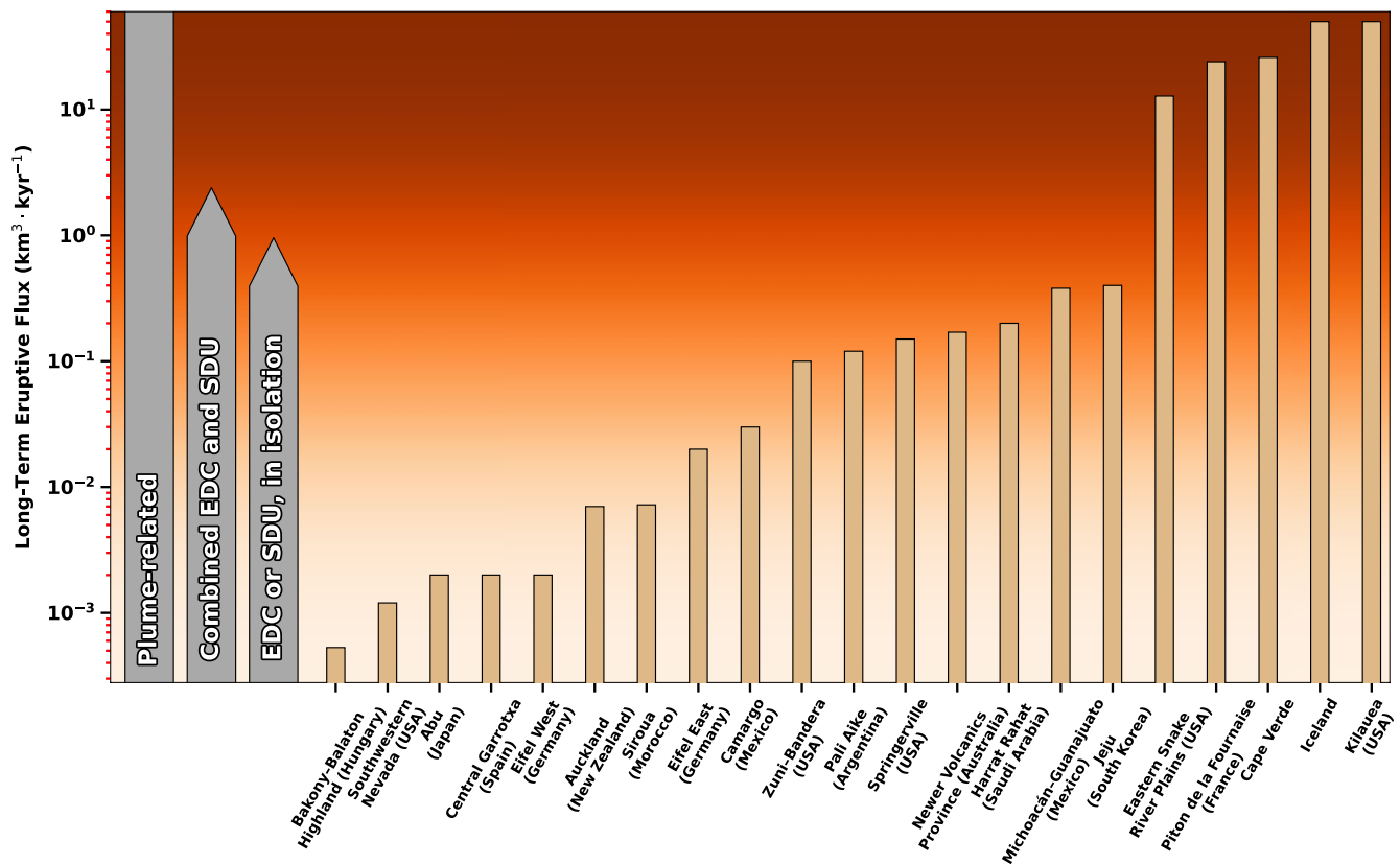
Figure 12. Long-term eruptive flux for a selection of intraplate volcanic fields (building on van den Hove et al., 2017). Vertical gray arrows indicate the expected long-term flux that can be accounted for by given melt-generating mechanisms; we infer that mantle plumes are required to explain the largest fluxes observed. Values for province fluxes are taken from van den Hove et al. (2017), or as follows: Kilauea (Dvorak & Dzursin, 1993), Iceland (Thordarson & Höskuldsson, 2008), Piton de la Fournaise (Roult et al., 2012), Cape Verde (Holm et al., 2008), Siroua (Missenard & Cadoux, 2012).
