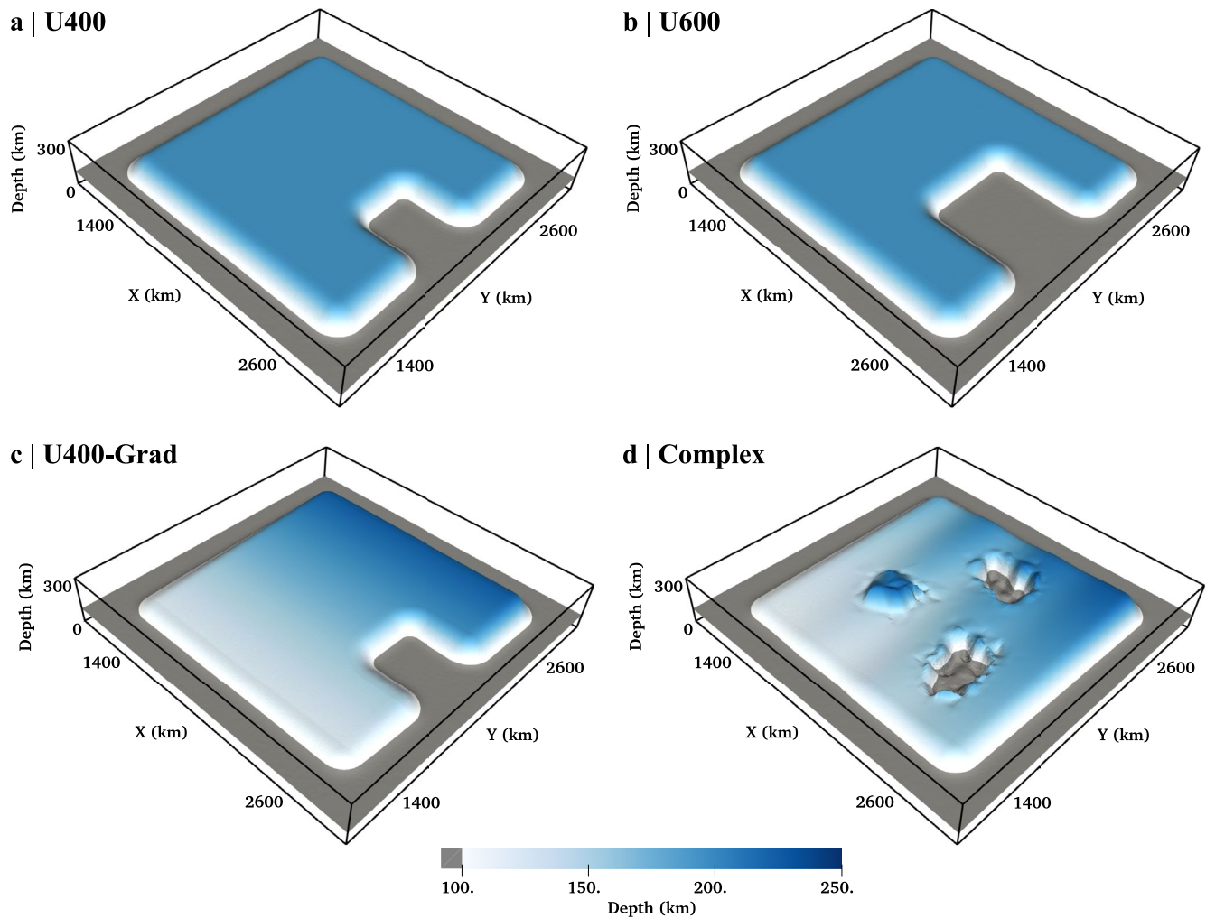
Figure 2. Initial topography of the LAB, as delineated by the 1,620 K isotherm, for continental geometries used in our 3-D simulations. On each panel, the view is from below, looking at the base of the continent. (a) Case U400. (b) Case U600. (c) Case U400-Grad. (d) Case Complex.
