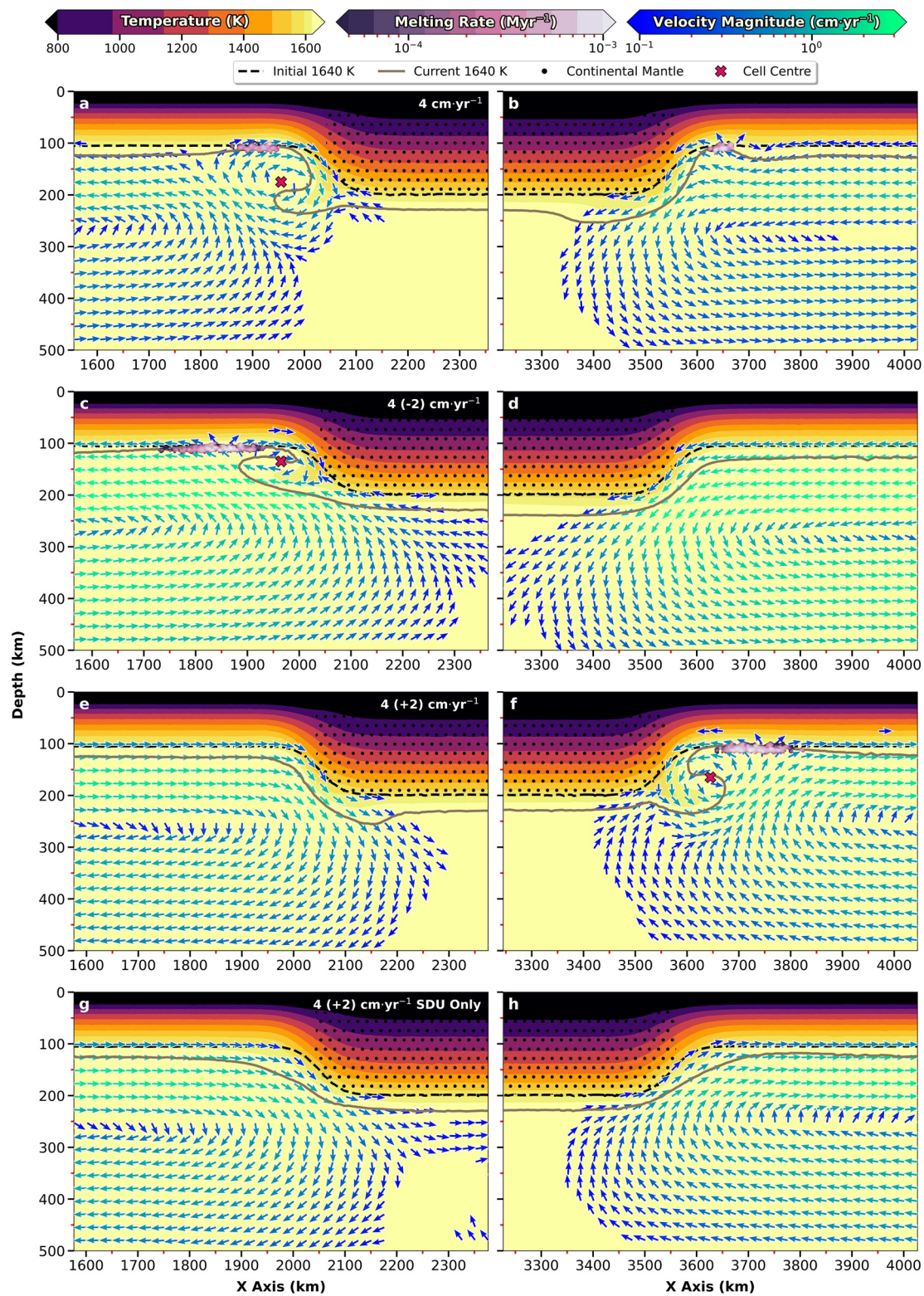
Figure 4. Effect of asthenospheric flow on edge-related dynamics. (a) and (b) 4 \text{ cm yr}^{-1} purely plate-driven scenario. (c) and (d) A case with additional shear in the asthenosphere, directed opposite to plate motion. (e) and (f) Similar to (c) and (d), but with asthenospheric shear aligned with plate motion direction. (g) and (h) Similar to (e) and (f), but with the coefficient of thermal expansion set to 0, thus negating edge-driven instabilities. All models are displayed after 20 Myr of model evolution. Graphics illustration as in Figure 3, with the horizontal component of velocity relative to that of a vertical transect through the center of the continent.
