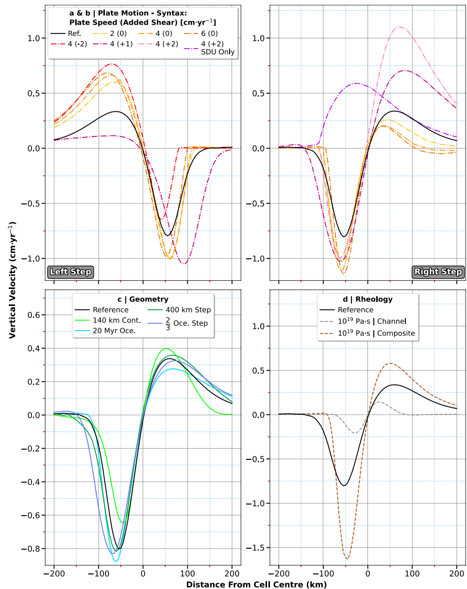
Figure 5. Comparison of vertical velocity in the vicinity of the cell center (see Figure S4 for computed locations) at the right step (if not specified) for the 2-D simulations examined herein. As instabilities develop over different time scales for different cases, we identify the center of the cell in each simulation (Figure S4) at the time of maximum downwelling velocity (Figure S5) prior to the onset of secondary instabilities, to provide a meaningful comparison. Each profile represents a 400 km horizontal transect passing through the center of the cell. (a) and (b) Influence of background asthenospheric flow, “Reference” corresponds to an enclosed simulation. At the right step, purely plate-driven cases do not develop a full circulating cell and, accordingly, velocity profiles are displayed at depths picked to allow for illustration of upwelling velocities in a way that is comparable to other cases. Moreover, the case with shear-driven upwelling (SDU) only does not generate a cell at all and we use the cell center from the equivalent case (“4 (+2)”) to draw the profile to allow for a representative comparison. (c) Effect of step geometry, “Reference” corresponds to “40 Myr Oce.”, “200 km Step”, “200 km Cont.”, and a material boundary halfway along the step. (d) Role of viscosity, “Reference” corresponds to a purely diffusion creep channel-free profile with a minimum viscosity of 10 19 Pa s.
