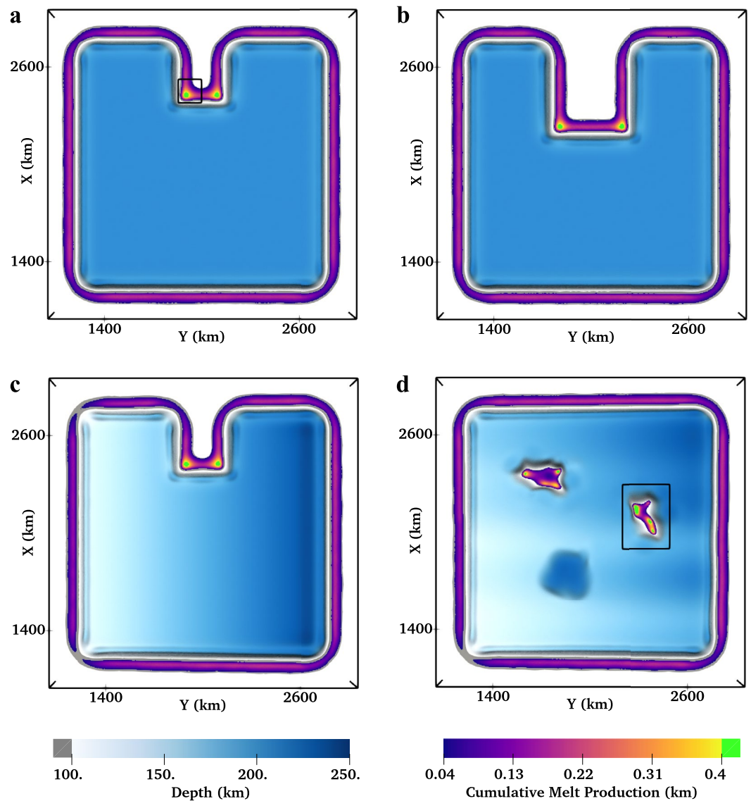
Figure 8. Cumulative melt production adjacent to the continent for cases without plate motion, after 15 Myr. Surface colors correspond to the depth of the 1,620 K isotherm, our proxy for lithospheric depth; lithospheric erosion is identified by the gray tone, which depicts portions thinner than 100 km. Purple-to-yellow colors represent the cumulative melt production as obtained after integration along the vertical axis (Section 2.4); major locations of melting are indicated by the green tone. Black rectangles illustrate zones of interest used for calculations in Table 3. (a) Case U400. (b) Case U600. (c) Case U400-Grad. (d) Case Complex.
