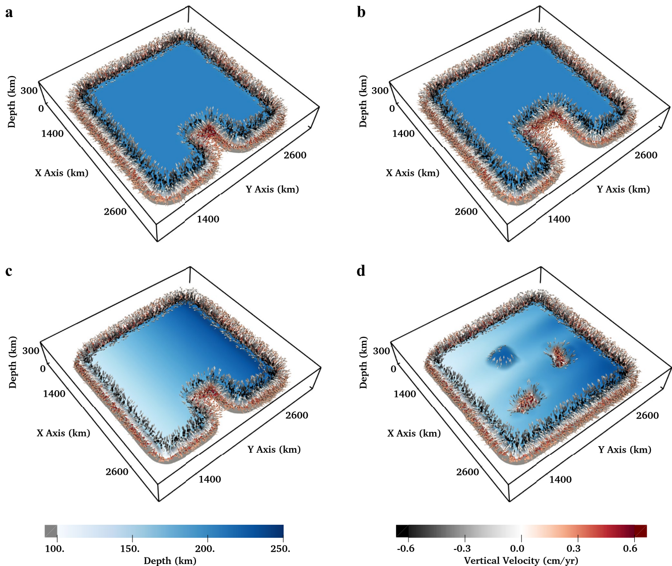
Figure 7. 3-D representation of the velocity field around the continent at 15 Myr, illustrated through a view looking at the base of the continent, from below. Surface colors correspond to the depth of the 1,620 K isotherm, our proxy for lithospheric thickness, while arrow glyphs illustrate the velocity field. For visualization purposes, glyphs are only drawn at locations where the velocity magnitude is larger than 2 \text{ mm yr}^{-1} ; glyphs all have the same length, are uniformly distributed and are colored according to the vertical component of velocity. (a) Case U400. (b) Case U600. (c) Case U400-Grad. (d) Case Complex.
