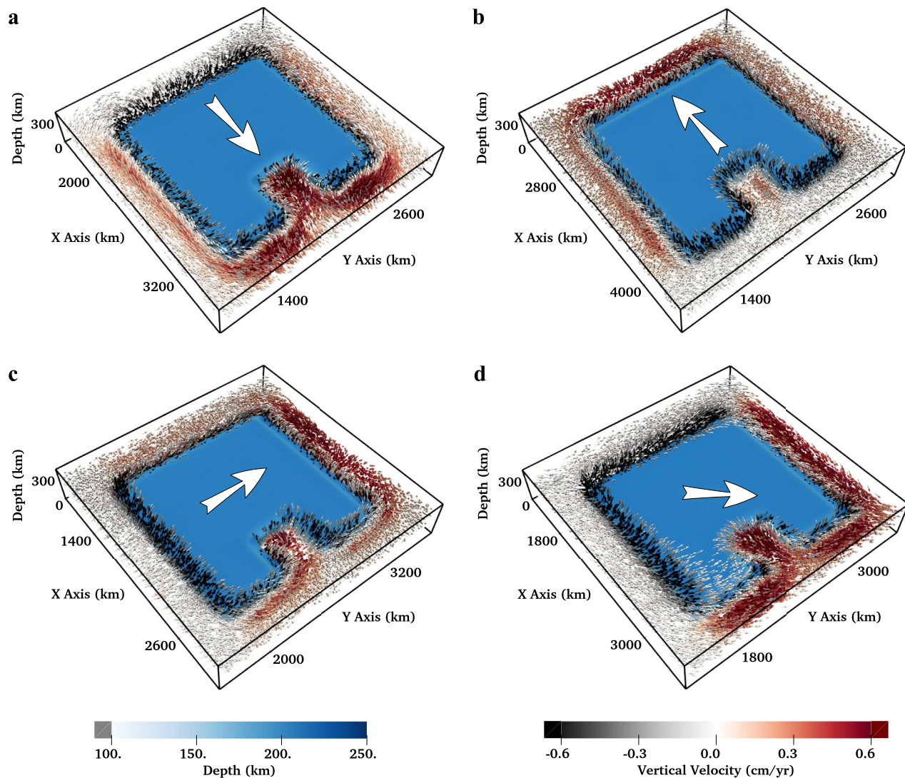
Figure 9. 3-D representation of the velocity field around the continental area after 15 Myr. Graphic illustration is similar to Figure 7; glyphs are only drawn where the velocity magnitude is greater than 4 \text{ mm yr}^{-1} . Similar to Figure 4, horizontal components of velocity are relative to that sampled on the vertical profile centered through the continent, uncovering dynamical instabilities. Additionally, large white arrows represent both the direction of plate motion and the direction of asthenospheric flow relative to the continent, thereby pointing from the continent's leading edge to its trailing edge. (a) Prescribed flow in the direction of positive x . (b) Direction of negative x . (c) Direction of positive y . (d) Direction of both positive x and y .
