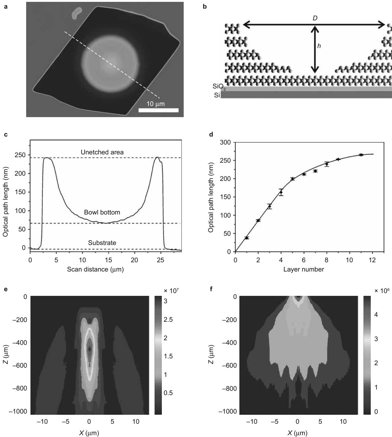
Figure 3 Atomically thin micro-lens fabricated from a few layers of MoS 2 . (a) PSI image of an atomically thin micro-lens fabricated on a 9L MoS 2 flake. (b) Schematic plot of the micro-lens structure. The bowl-shaped structure of the micro-lens was fabricated by FIB milling with atomic resolution in the vertical direction and sub-20 nm resolution in lateral direction. (c) Measured OPL values versus position for the direction indicated by the dashed line in (a) . (d) Measured statistical data of the OPL values for MoS 2 flakes with different layers ranging from 1L to 11L. For each layer number of MoS 2 , at least five different samples were characterized in the statistical measurements. All the layer numbers were confirmed by AFM. (e) Intensity distribution pattern of the MoS 2 micro-lens measured by scanning optical microscopy (SOM). (f) Intensity distribution pattern of the planar reference SiO 2 /Si substrate measured by the same SOM setup.
