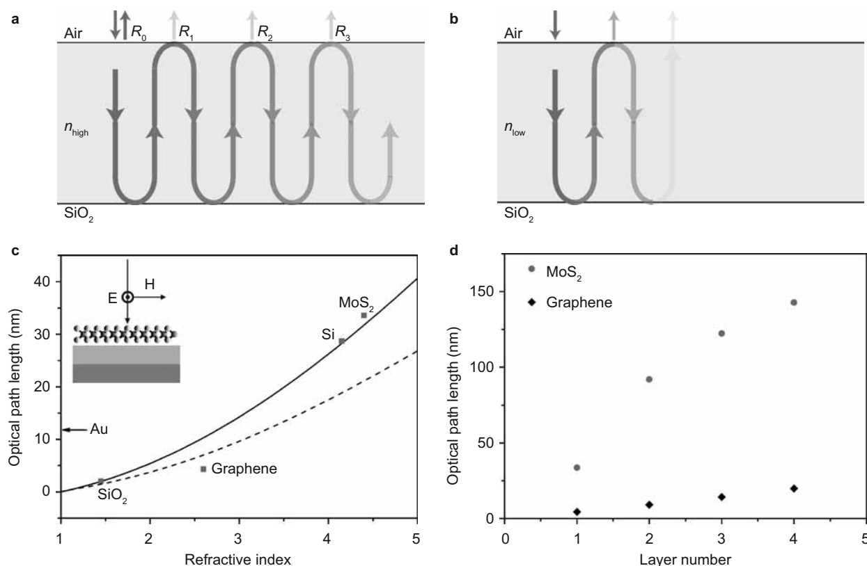
Figure 2 High refractive index enabled giant OPL in ultra-thin film. (a and b) Schematic plots of multiple reflections at the interfaces of ultra-thin 2D materials. High refractive index leads to a large reflection coefficient. Light is reflected many times inside the material and leads to a highly enhanced light path, indicated as (a). For low refractive index material, the light path is much less enhanced because of the small reflection coefficient, indicated as (b). (c) Simulated OPL values for light reflected from 2D material (0.67 nm in thickness) with different indices on a \text{SiO}_2 (275 nm)/Si substrate (solid line) and \text{SiO}_2 substrate with infinite thickness (dashed line). The calculated OPLs of 0.67 nm Au, 0.67 nm \text{SiO}_2 , 1L (0.34 nm) graphene, and 1L (0.67 nm) \text{MoS}_2 are represented by markers. (d) Simulated OPL values for 1L, 2L, 3L, and 4L \text{MoS}_2 and graphene on \text{SiO}_2 (275 nm)/Si substrate, respectively. The wavelength used in the simulations was 535 nm.
