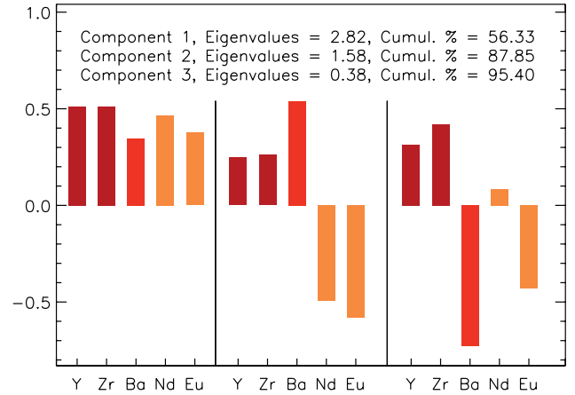
Figure 11. The composition of the first three normalized principal components for the n-capture elements for the high-metallicity sample.
