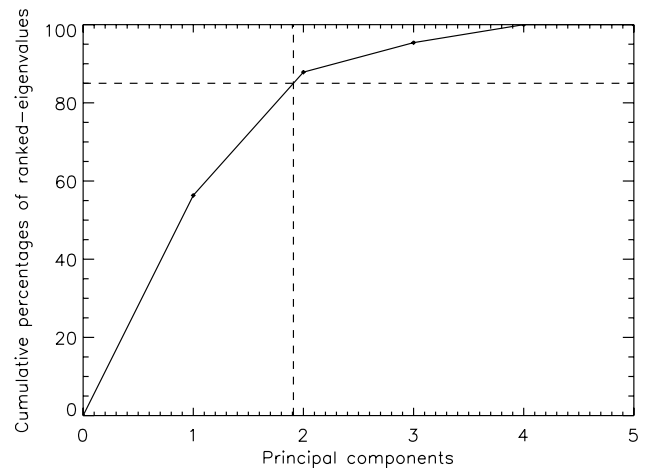
Figure 12. The ranked-eigenvalues cumulative percentages for the n-capture elements for the high-metallicity sample.
