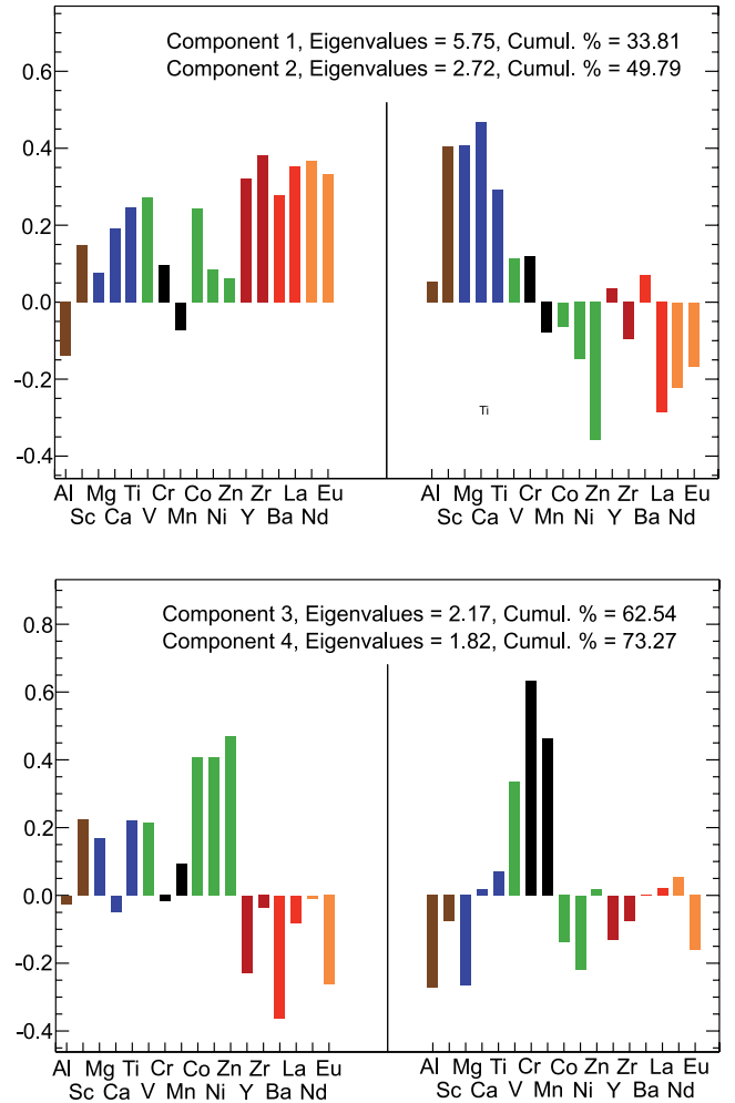
Figure 8. The normalized principal components of 17 elements for the low-metallicity sample (Barklem et al. 2005). [Al/Fe] is corrected for NLTE effect with +0.6 dex. The upper plot and lower plot show the first two principal components and the third and fourth principal components, respectively.
