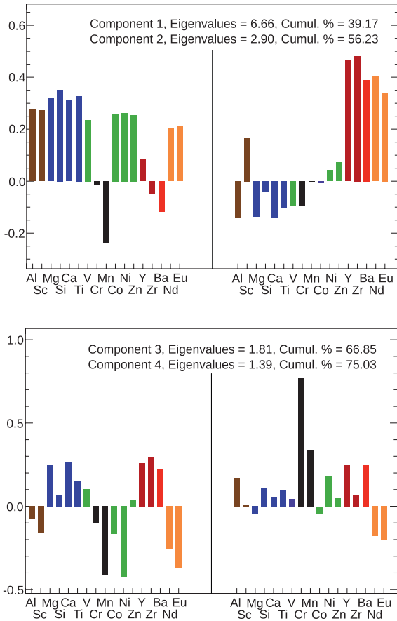
Figure 13. The normalized principal components of 17 elements for the high-metallicity sample. The upper and lower plots show the first two principal components and the third and fourth principal components, respectively.
