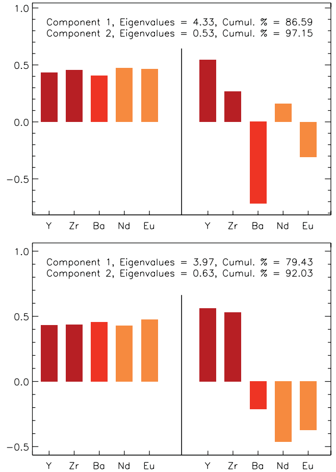
Figure 6. The composition of the first two n-capture elements normalized principal components, i.e. the eigenvector components of the n-capture elements correlation matrix, using the low-metallicity samples: Barklem's sample (upper plot) and First Stars Survey sample (lower plot). The horizontal axis shows the five n-capture elements and the vertical axis shows the component of the eigenvector in the direction of each of the five elements. See the text for the colour code.
