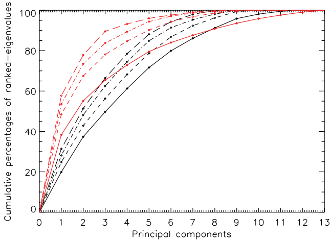
Figure 16. The same as Fig. 15 but for 13 elements, and assuming measurement uncertainty of 0.05, 0.07 and 0.20 dex, respectively, for open clusters, and 0.03, 0.05 and 0.10 dex, respectively, for solar neighbourhood stars.
