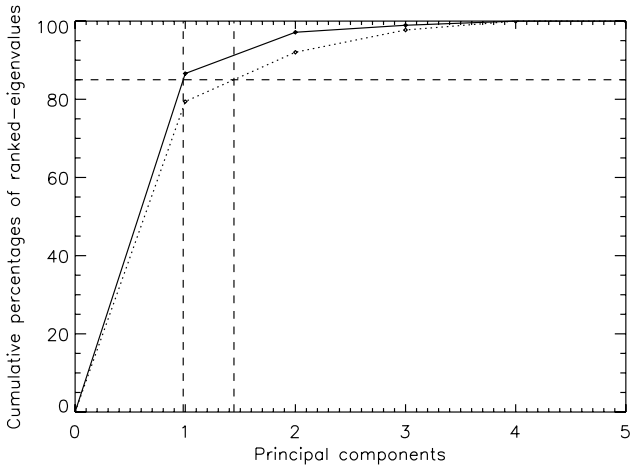
Figure 5. This ranked-eigenvalues cumulative percentages of n-capture elements (Y, Zr, Ba, Nd and Eu) for the low-metallicity samples: Barklem et al. (2005) sample (solid line) and First Stars Survey sample (dotted line).
