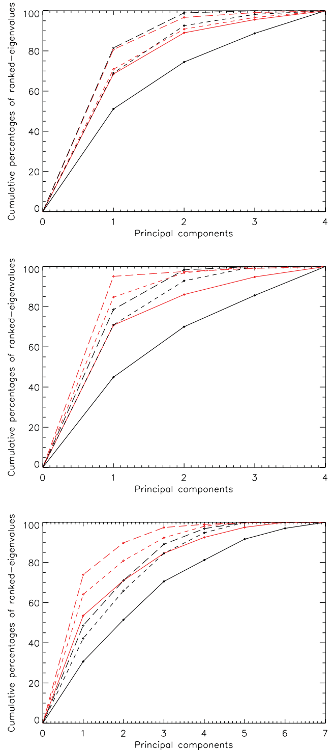
Figure 21. The ranked-eigenvalues cumulative percentages for the globular clusters (black lines) and the solar neighbourhood stars (red lines) in the same metallicity range: n -capture elements (upper panel), \alpha -elements (middle panel) and all elements in common (lower panel). The solid lines show the observed correlation. The dashed/broken lines show the cumulative percentages derived from the estimated intrinsic correlation matrix, assuming measurement uncertainty of 0.1, 0.2 dex, respectively, for globular clusters, and 0.05, 0.1 dex, respectively, for the solar neighbourhood stars.
