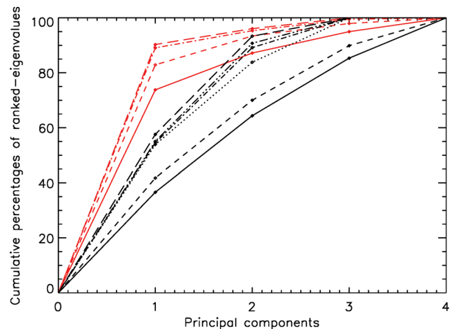
Figure 15. The ranked-eigenvalues cumulative percentages of the \alpha -elements, comparing open clusters (black lines) with solar neighbourhood stars (red lines). The solid lines show the observed correlation. The dashed/broken lines show the cumulative percentages derived from the estimated intrinsic correlation matrix, assuming measurement uncertainty of 0.05, 0.07, 0.10, 0.15 and 0.20 dex, respectively, for open clusters, and 0.02, 0.03 and 0.10 dex, respectively, for solar neighbourhood stars.
