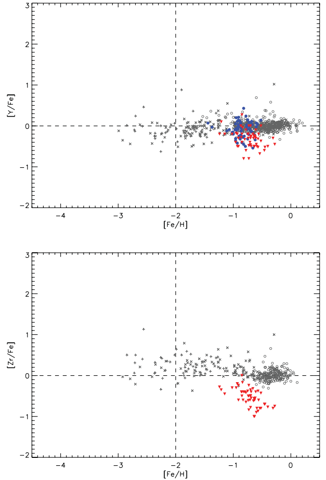
Figure 23. The [ls/Fe] – [Fe/H] of the solar neighbourhood, Fornax and the LMC stars. The symbols are the same as in Fig. 22. The two dwarf galaxies have similar or lower abundances of ls elements compared to solar neighbourhood stars.
