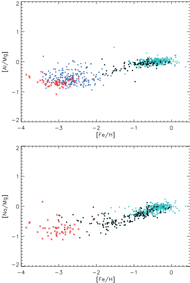
Figure 25. These plots show the ratio of light odd-Z elements (Al and Na) to light even-Z elements/ \alpha -elements (Mg) as a function of [\text{Fe}/\text{H}] of solar neighbourhood halo and disc stars. The symbols are the same as in Fig. 7. Al, Na and Mg abundances for First Stars Survey are NLTE corrected according to Andrievsky et al. (2007, 2008, 2010) in these two plots. [\text{Al}/\text{Fe}] for Barklem’s sample are NLTE corrected by +0.6 dex. Both plots show an odd–even effect, i.e. light odd-Z elements are suppressed at low metallicity.
