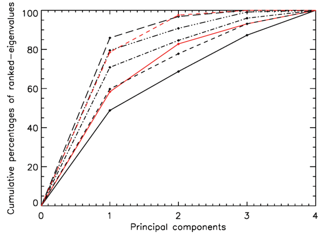
Figure 17. The n-capture element ranked-eigenvalues cumulative percentages comparing the Fornax dSph galaxy (black lines) with its solar neighbourhood counterparts (red lines) in the same metallicity range. The solid lines show the observed correlation. The dashed/broken lines show the cumulative percentages derived from the estimated intrinsic correlation matrix, assuming measurement uncertainty of 0.1, 0.13, 0.15 and 0.2 dex, respectively, for the dSph, and 0.07 dex for the solar neighbourhood counterparts.
