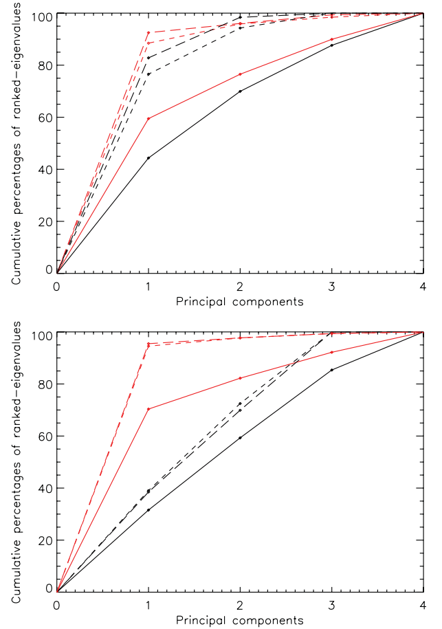
Figure 19. The ranked-eigenvalues cumulative percentages for the \alpha -elements for the dwarf galaxies (black lines) and the solar neighbourhood (red lines) in the same metallicity range. The results for Fornax and the LMC are shown in the upper plot and lower plot, respectively. The solid lines show the observed correlation. The dashed/broken lines show the cumulative percentages derived from the estimated intrinsic correlation matrix, assuming measurement uncertainty of 0.1, 0.15 dex, respectively, for the dwarf galaxies and 0.05, 0.1 dex, respectively, for the solar neighbourhood counterparts.
