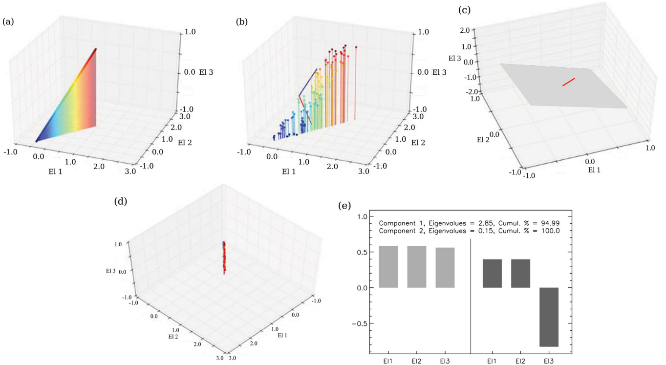
Figure 2. This is a model ( \gamma = 1 ) to illustrate how PCA works. The vertical lines in panels (a) and (b) are visual guides. Panel (a) shows the scatter plot of the chemical abundances where only mechanism 1 is working (see text). Panel (b) is the same as (a) but both mechanisms 1 and 2 are contributing to the chemical abundances. Panel (b) also shows the first principal component in blue solid line and the second principal component in red solid line. Panel (c) shows the hyperplane of the first principal component in grey and the second principal component in red solid line. Panel (d) shows the data points projected on to the hyperplane of the first principal component and the red solid line is the second principal component. Panel (e) shows the composition of the first two normalized eigenvectors. Colour version of all figures in this paper is available in the online version of the journal.
