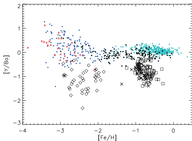
Figure 24. The Y ( Is ) to Ba ( hs ) ratios as a function of [Fe/H] for solar neighbourhood not-CEMP stars, CEMP-s stars and dwarf galaxies stars. The solar neighbourhood not-CEMP stars symbols are the same as in Fig. 7. CEMP-s stars are plotted with black open diamonds. Fornax stars are plotted with black crosses and the LMC stars are plotted with black open squares.
