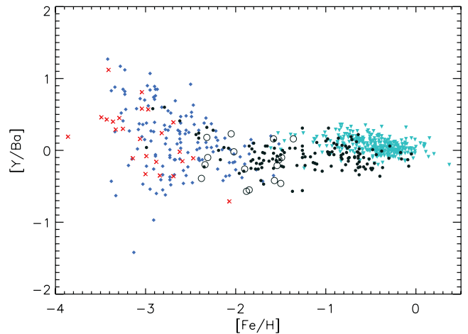
Figure 7. Y ( ls ) to Ba ( hs ) ratios as a function of [Fe/H] for the Milky Way halo/disc stars from First Stars Survey (red crosses), Barklem et al. (2005) (blue diamonds), Fulbright (2000, 2002) (black filled circles), Reddy et al. (2003, 2006) (cyan triangles) and globular clusters from Pritzl et al. (2005) (black open circles) All samples assume 1D-LTE stellar model.
