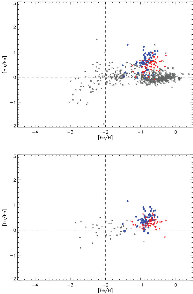
Figure 22. The [hs/Fe] – [Fe/H] of the solar neighbourhood, Fornax and the LMC stars. The symbols in grey represent the solar neighbourhood compilation from Burris et al. (2000) (plus), Fulbright (2000, 2002) (crosses) and Reddy et al. (2003, 2006) (open circles). The blue filled circles are Fornax stars from Letarte et al. (2010). The red filled triangles are the LMC stars from Pompeia et al. (2008). The two dwarf galaxies are overabundant in hs elements, compared to solar neighbourhood stars.
