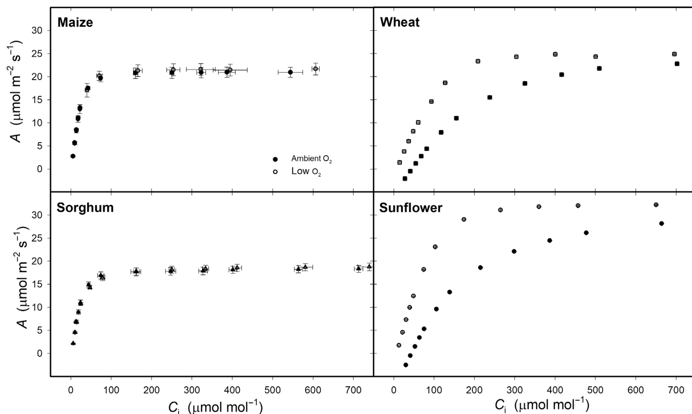
Fig. 2 Response of assimilation to \text{CO}_2 concentration in the substomatal cavity ( A/C_i curves). Responses were measured under ambient \text{O}_2 concentration (filled symbols) or under low \text{O}_2 concentration (empty symbols) at a light intensity of 500 \mu\text{mol m}^{-2} \text{s}^{-1} , on fully hydrated maize (top left), wheat (top right), sorghum (bottom left), or sunflower (bottom right) leaves. n = 4 biological replicates for each species. Error bars show \pm SE for A and C_i .
