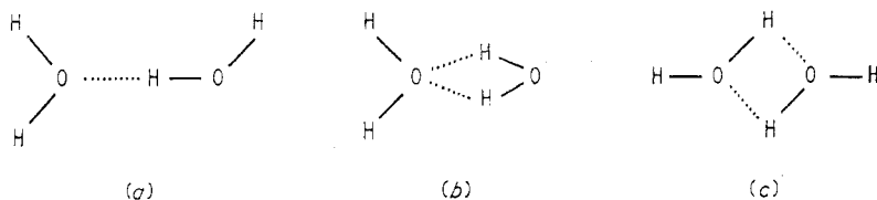
Figure 6. Possible equilibrium configurations for the water dimer: (a) linear, (b) bifurcated and (c) cyclic.
