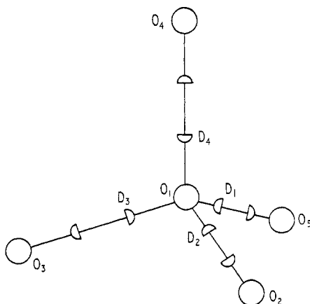
Figure 13. The nearest-neighbour environment of a molecule in D_2O ice showing the half-deuteron positions.
