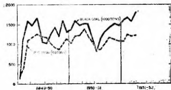
PRODUCTION OF BLACK COAL AND PIG IRON
