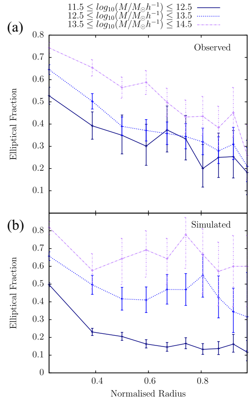
Figure 8. The elliptical fraction for three group mass bins ( 10^{12} , 10^{13} , 10^{14} M_{\odot} , solid, dashed and dot-dashed lines, respectively) for the observed GAMA groups (top panel) and simulation groups (bottom panel). The radii in each group are all normalized to the radius containing all the group members. The error bars denote the 95 per cent binomial confidence intervals. The elliptical fraction peaks at the centre in both observed and simulated groups.
