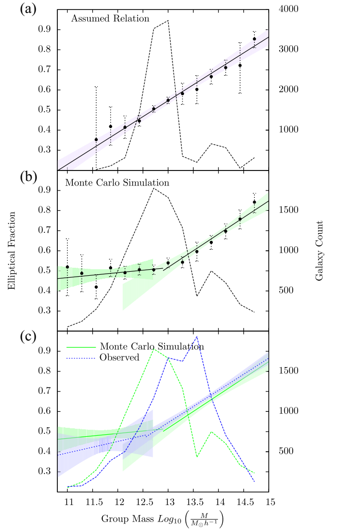
Figure 4. The effect of uncertainty in group masses on the group mass morphology relation. (a) The elliptical galaxy fraction for one simulation of our survey assuming a constant linear relation over the whole range of group mass. No uncertainties have been added to the group masses. (b) The resulting group mass–morphology relation after adding uncertainties to the group masses. (c) The group mass–morphology relation from (b) (green, solid lines) overlaid by the observed relation found in Fig. 3 (blue, dotted lines). Dotted curves show the number of galaxies in each bin. Shaded areas are the 95 per cent confidence bounds for the linear regressions. The reintroduction of mass uncertainties to (a) reproduces the flattening seen below 10^{12.5} M_{\odot} in the observational result while maintaining the original gradient at higher masses.
